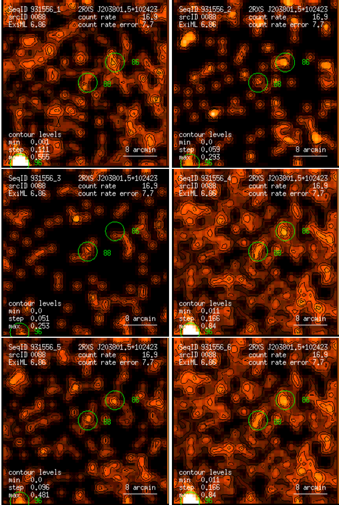
Figure 88: RASS 931556: detection 0088: band rate images, Gaussian filter: (1) PSPC channels 11 – 41, (2) 52 – 90, (3) 91 – 201, (4) 11 – 235, (5) 52 – 201, (6) 11 – 201. Broad band rates in counts/ks. Band rate contour levels in counts/ks/arcmin 2 .
