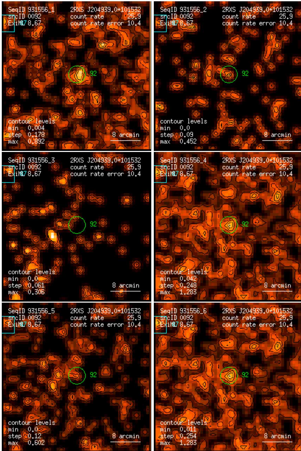
Figure 92: RASS 931556: detection 0092: band rate images, Gaussian filter: (1) PSPC channels 11 – 41, (2) 52 – 90, (3) 91 – 201, (4) 11 – 235, (5) 52 – 201, (6) 11 – 201. Broad band rates in counts/ks. Band rate contour levels in counts/ks/arcmin 2 .
