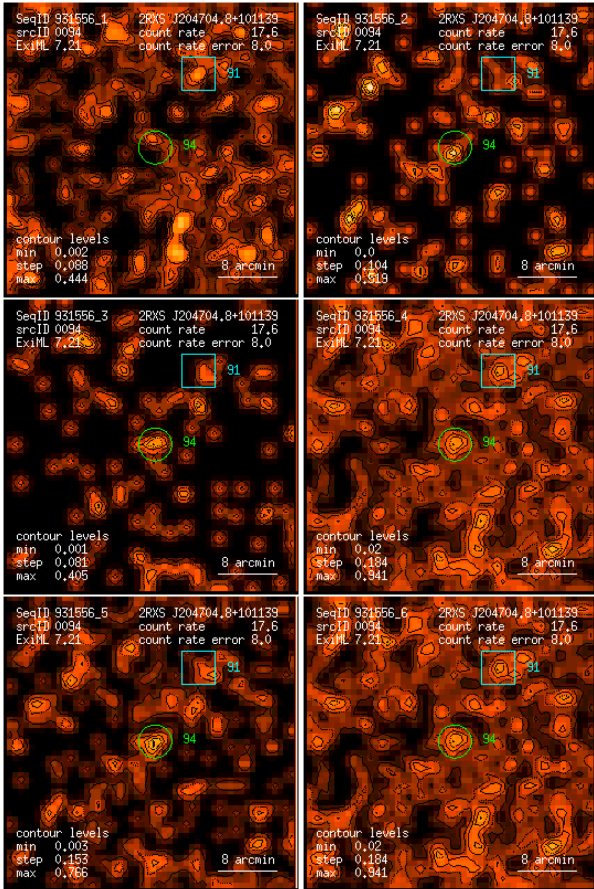
Figure 94: RASS 931556: detection 0094: band rate images, Gaussian filter: (1) PSPC channels 11 – 41, (2) 52 – 90, (3) 91 – 201, (4) 11 – 235, (5) 52 – 201, (6) 11 – 201. Broad band rates in counts/ks. Band rate contour levels in counts/ks/arcmin 2 .
