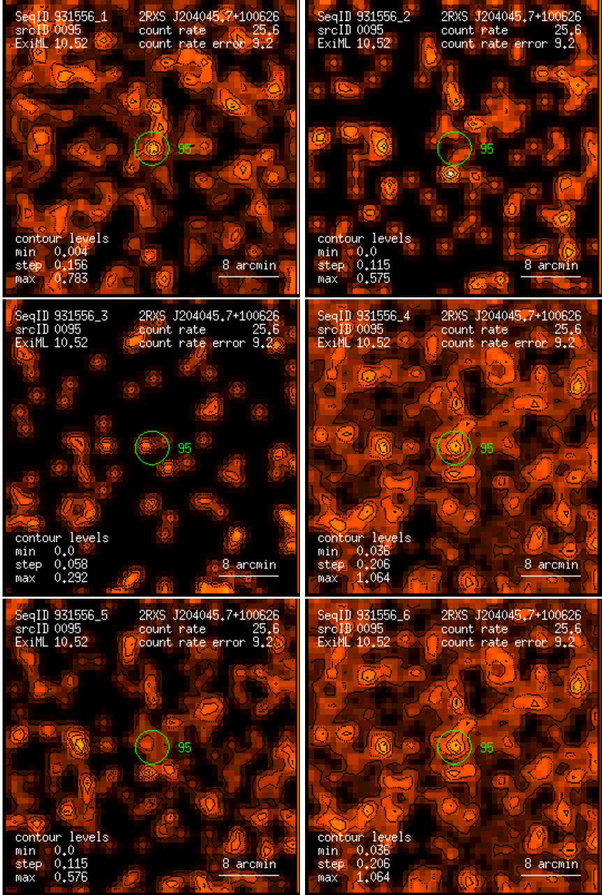
Figure 95: RASS 931556: detection 0095: band rate images, Gaussian filter: (1) PSPC channels 11 – 41, (2) 52 – 90, (3) 91 – 201, (4) 11 – 235, (5) 52 – 201, (6) 11 – 201. Broad band rates in counts/ks. Band rate contour levels in counts/ks/arcmin 2 .
