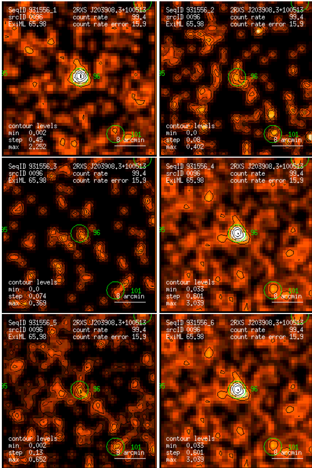
Figure 96: RASS 931556: detection 0096: band rate images, Gaussian filter: (1) PSPC channels 11 – 41, (2) 52 – 90, (3) 91 – 201, (4) 11 – 235, (5) 52 – 201, (6) 11 – 201. Broad band rates in counts/ks. Band rate contour levels in counts/ks/arcmin 2 .
