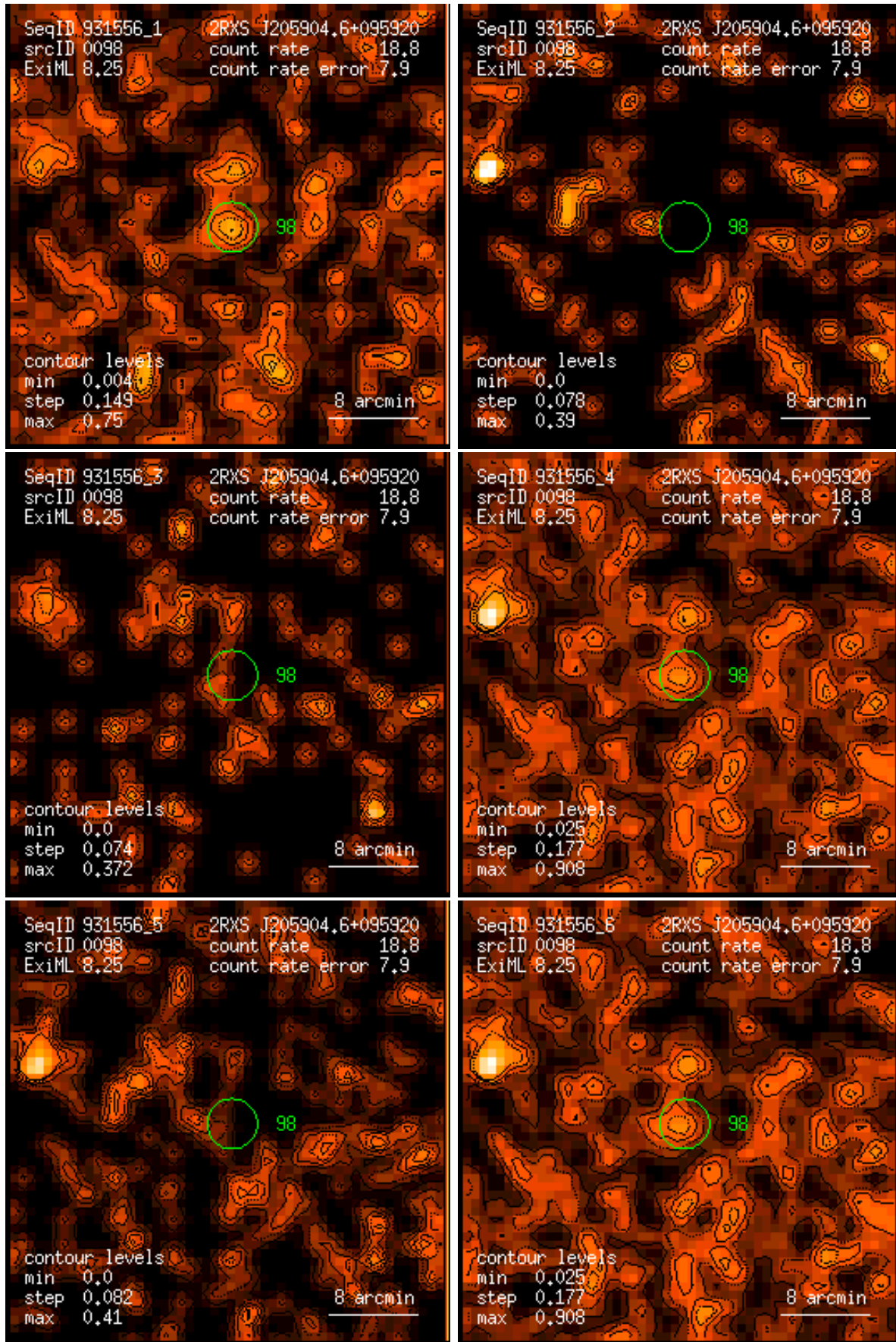
Figure 98: RASS 931556: detection 0098: band rate images, Gaussian filter: (1) PSPC channels 11 – 41, (2) 52 – 90, (3) 91 – 201, (4) 11 – 235, (5) 52 – 201, (6) 11 – 201. Broad band rates in counts/ks. Band rate contour levels in counts/ks/arcmin 2 .
