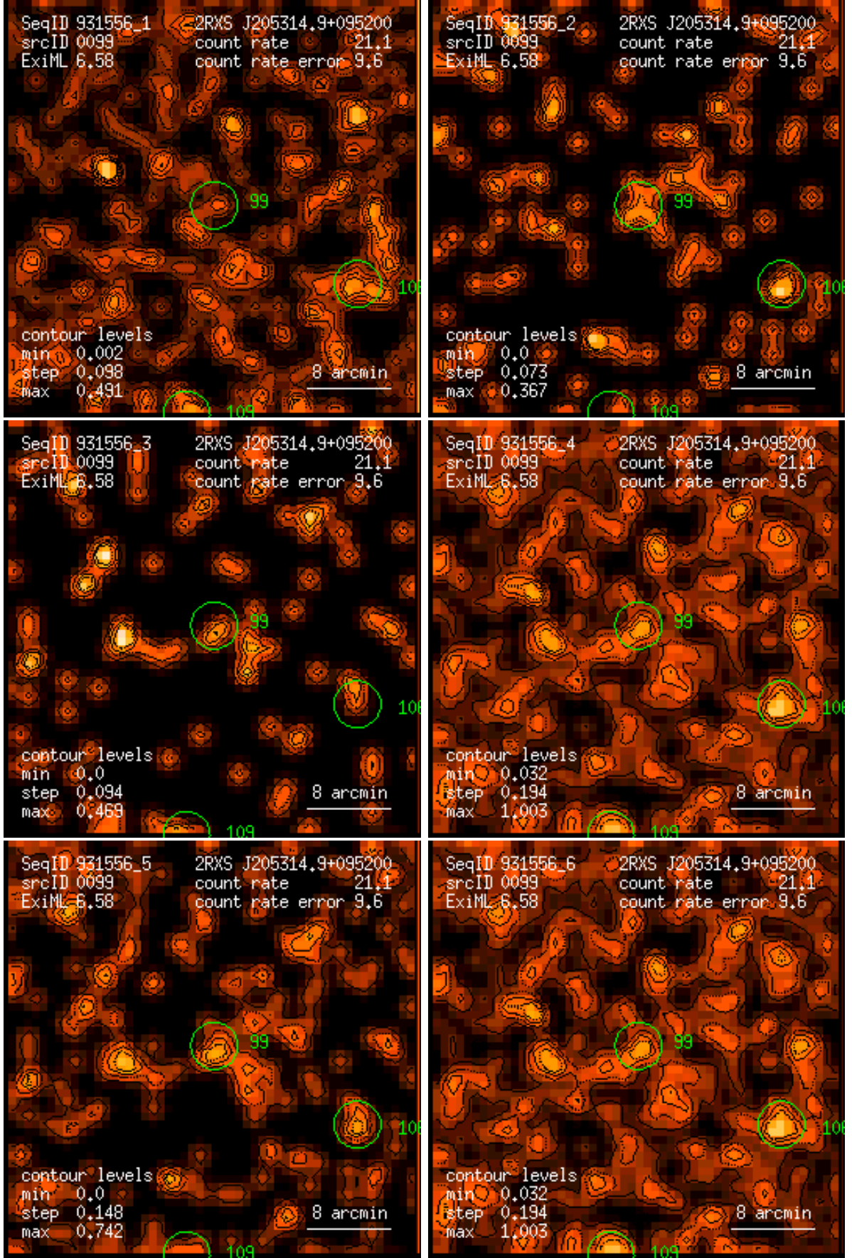
Figure 99: RASS 931556: detection 0099: band rate images, Gaussian filter: (1) PSPC channels 11 – 41, (2) 52 – 90, (3) 91 – 201, (4) 11 – 235, (5) 52 – 201, (6) 11 – 201. Broad band rates in counts/ks. Band rate contour levels in counts/ks/arcmin 2 .
