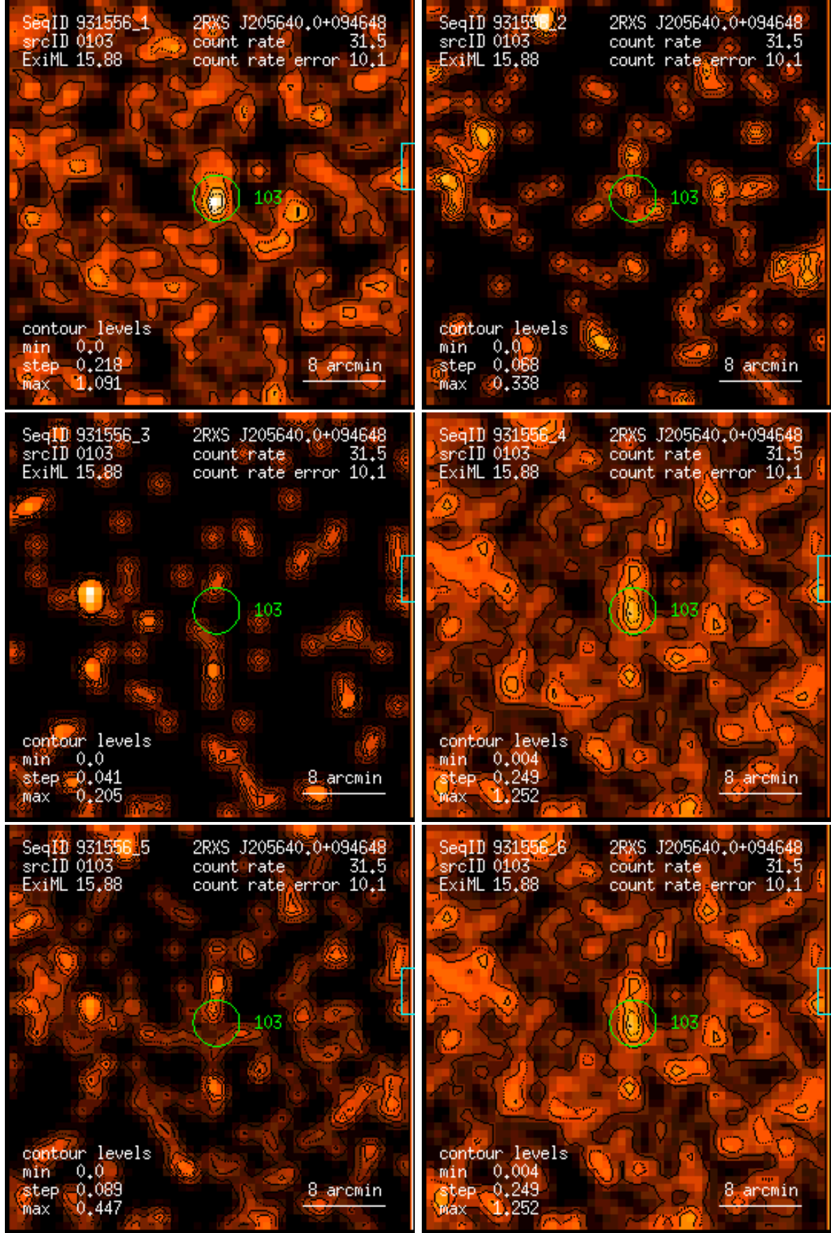
Figure 103: RASS 931556: detection 0103: band rate images, Gaussian filter: (1) PSPC channels 11 – 41, (2) 52 – 90, (3) 91 – 201, (4) 11 – 235, (5) 52 – 201, (6) 11 – 201. Broad band rates in counts/ks. Band rate contour levels in counts/ks/arcmin 2 .
