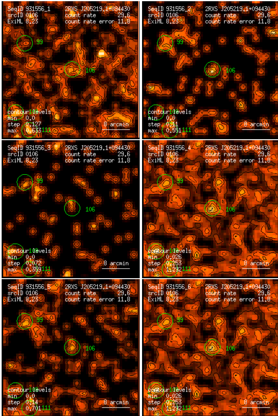
Figure 106: RASS 931556: detection 0106: band rate images, Gaussian filter: (1) PSPC channels 11 – 41, (2) 52 – 90, (3) 91 – 201, (4) 11 – 235, (5) 52 – 201, (6) 11 – 201. Broad band rates in counts/ks. Band rate contour levels in counts/ks/arcmin 2 .
