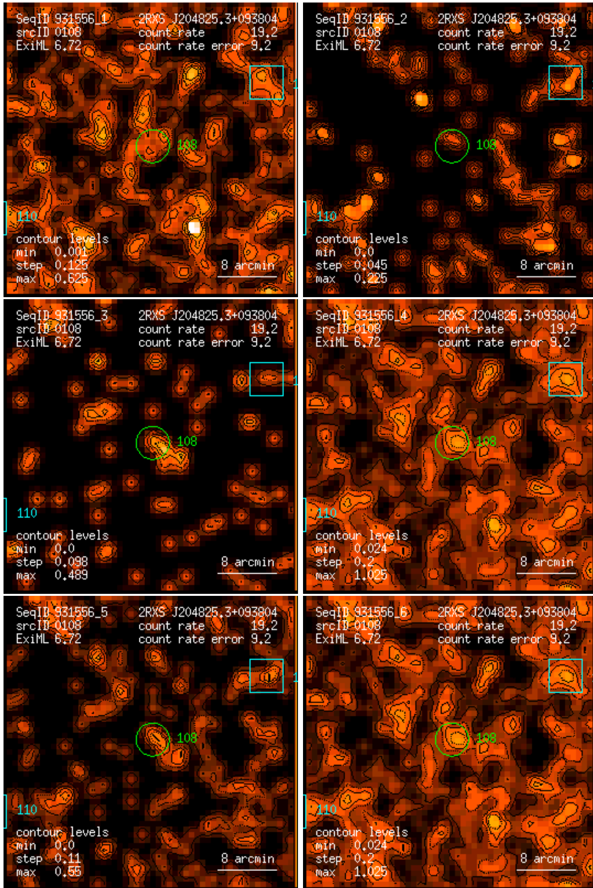
Figure 108: RASS 931556: detection 0108: band rate images, Gaussian filter: (1) PSPC channels 11 – 41, (2) 52 – 90, (3) 91 – 201, (4) 11 – 235, (5) 52 – 201, (6) 11 – 201. Broad band rates in counts/ks. Band rate contour levels in counts/ks/arcmin 2 .
