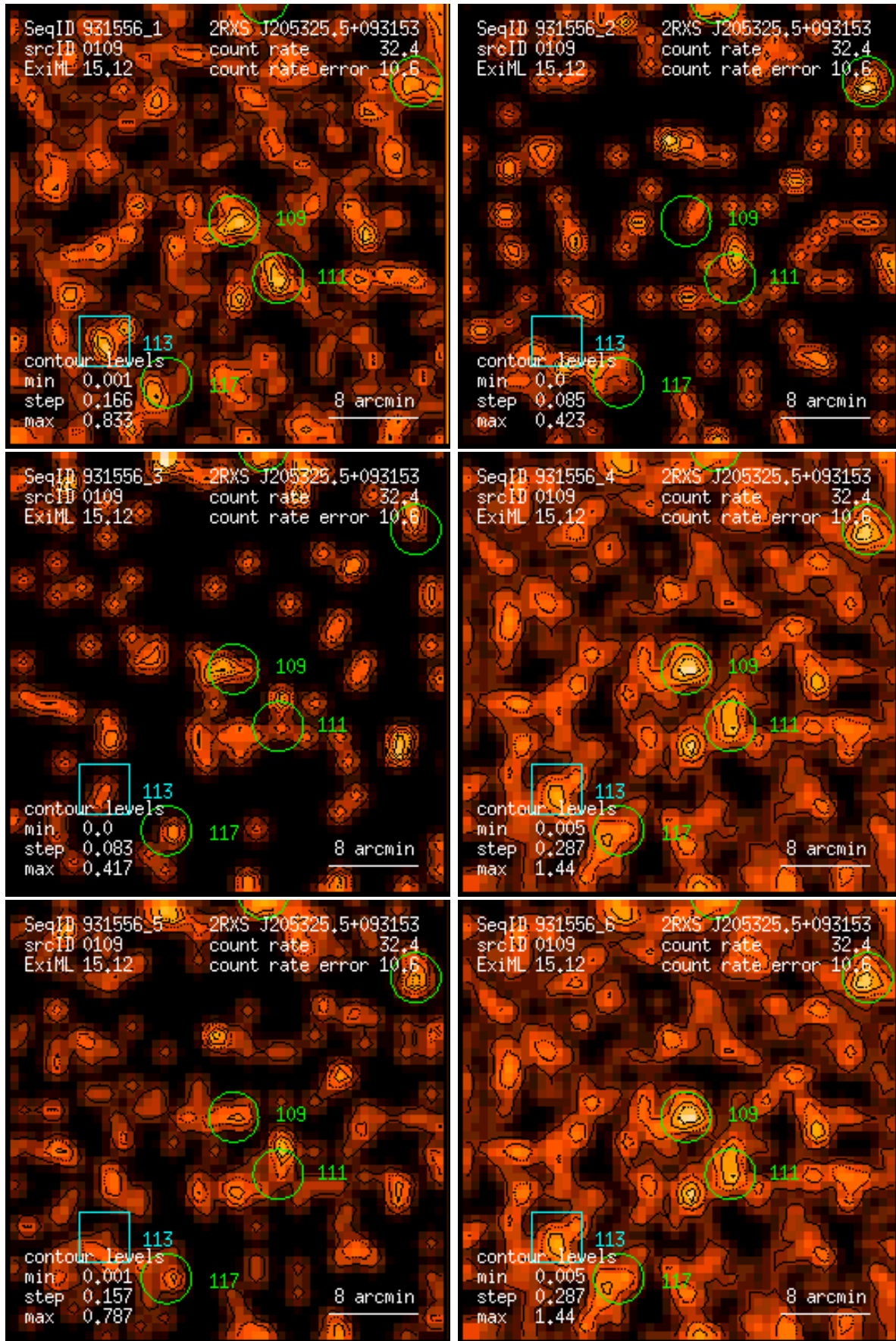
Figure 109: RASS 931556: detection 0109: band rate images, Gaussian filter: (1) PSPC channels 11 – 41, (2) 52 – 90, (3) 91 – 201, (4) 11 – 235, (5) 52 – 201, (6) 11 – 201. Broad band rates in counts/ks. Band rate contour levels in counts/ks/arcmin 2 .
