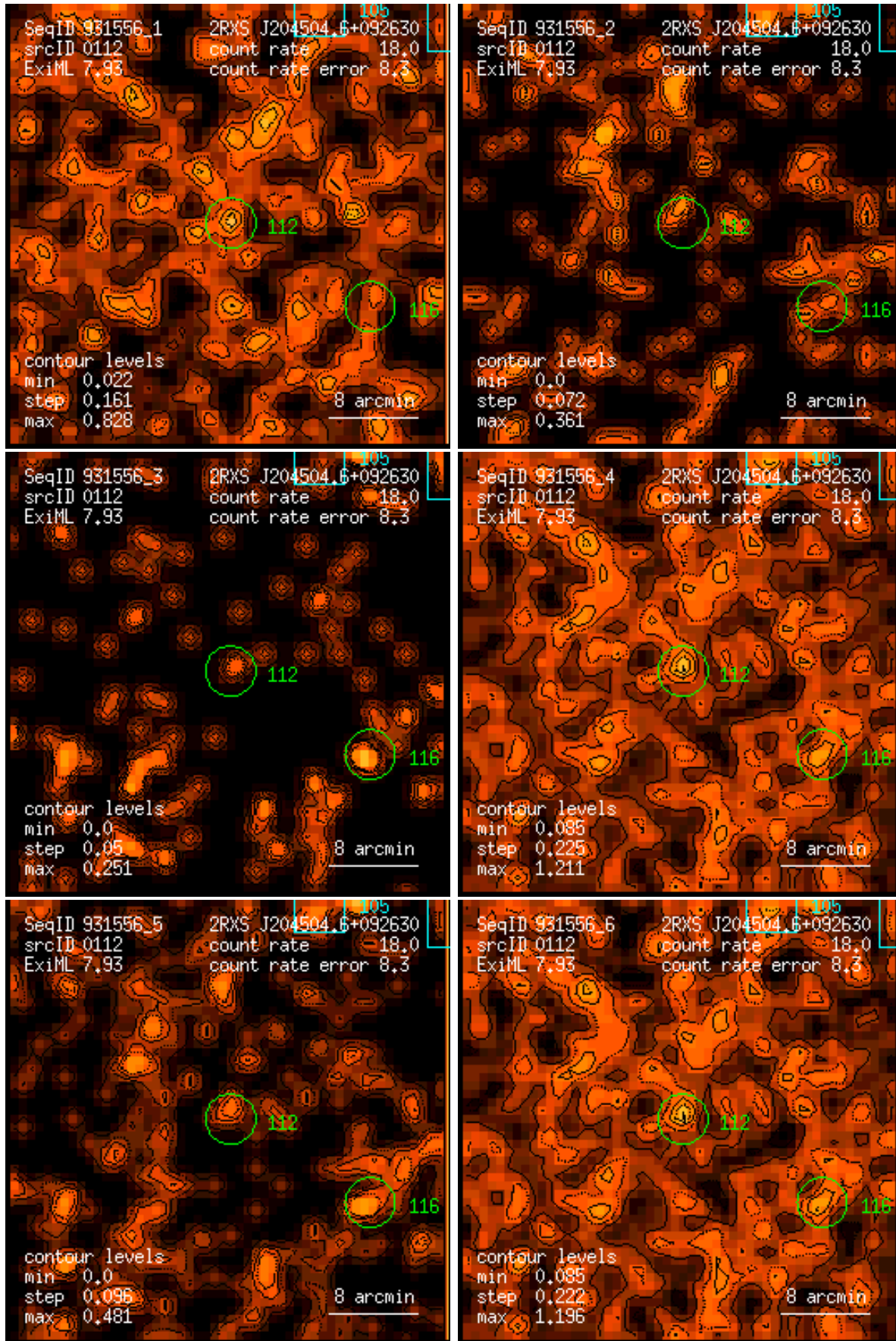
Figure 112: RASS 931556: detection 0112: band rate images, Gaussian filter: (1) PSPC channels 11 – 41, (2) 52 – 90, (3) 91 – 201, (4) 11 – 235, (5) 52 – 201, (6) 11 – 201. Broad band rates in counts/ks. Band rate contour levels in counts/ks/arcmin 2 .
