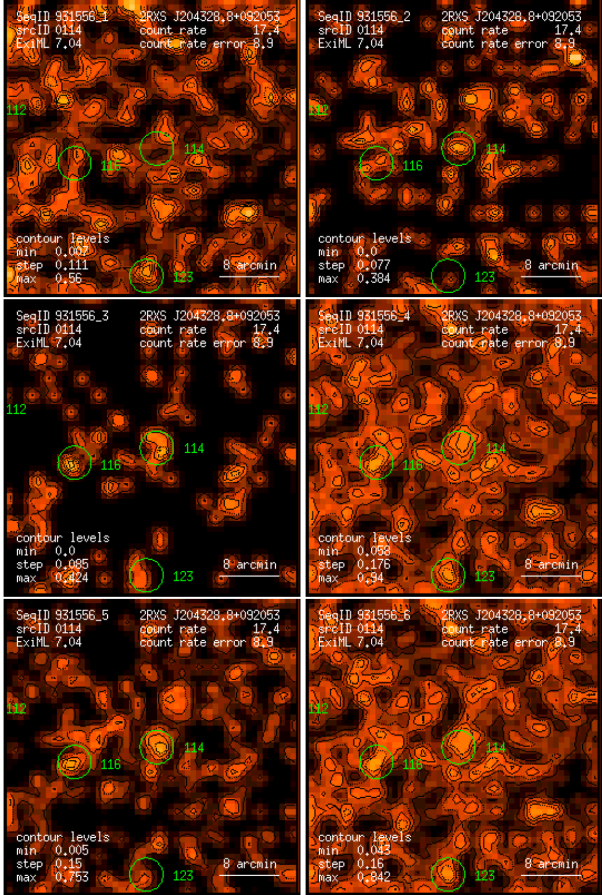
Figure 114: RASS 931556: detection 0114: band rate images, Gaussian filter: (1) PSPC channels 11 – 41, (2) 52 – 90, (3) 91 – 201, (4) 11 – 235, (5) 52 – 201, (6) 11 – 201. Broad band rates in counts/ks. Band rate contour levels in counts/ks/arcmin 2 .
