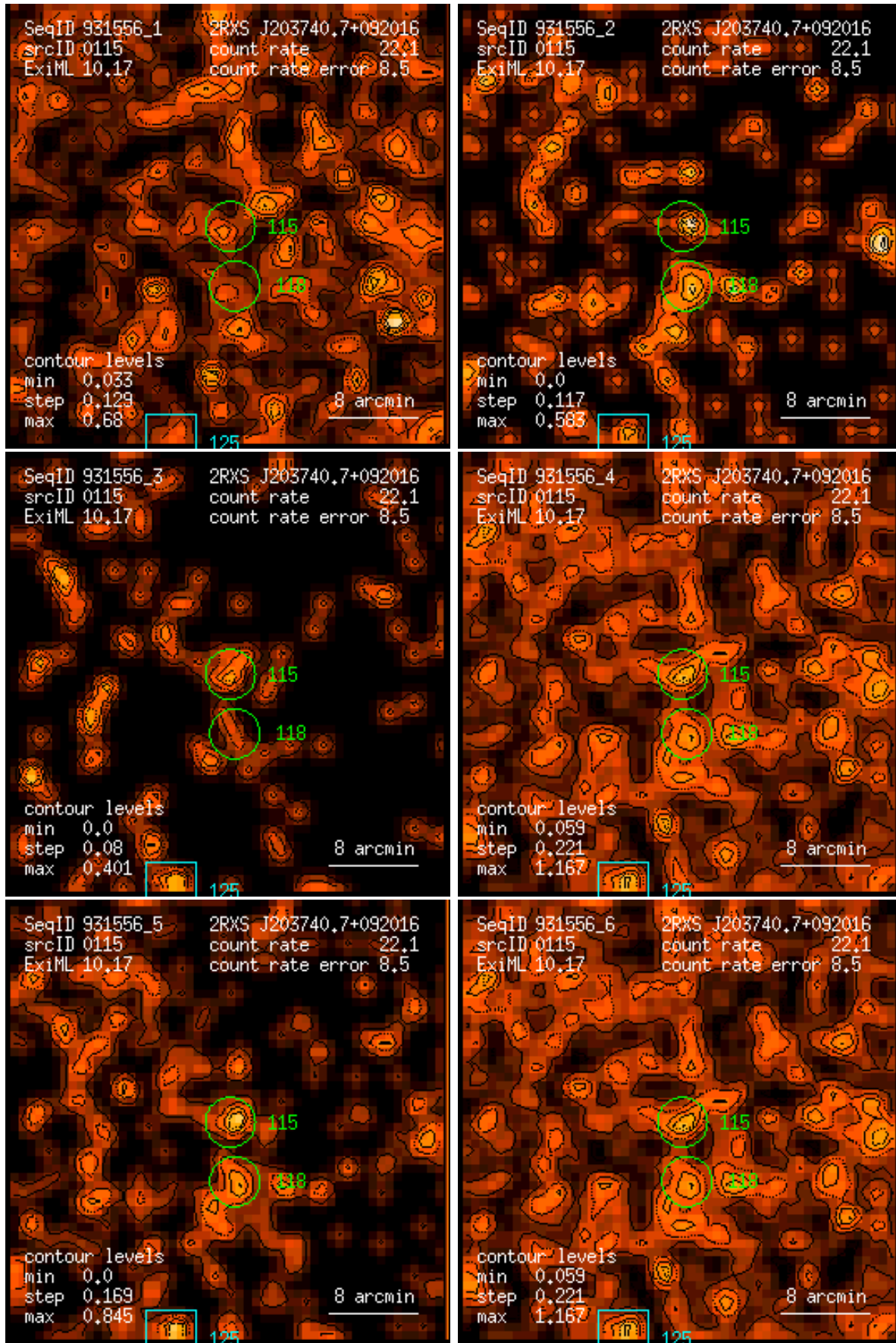
Figure 115: RASS 931556: detection 0115: band rate images, Gaussian filter: (1) PSPC channels 11 – 41, (2) 52 – 90, (3) 91 – 201, (4) 11 – 235, (5) 52 – 201, (6) 11 – 201. Broad band rates in counts/ks. Band rate contour levels in counts/ks/arcmin 2 .
