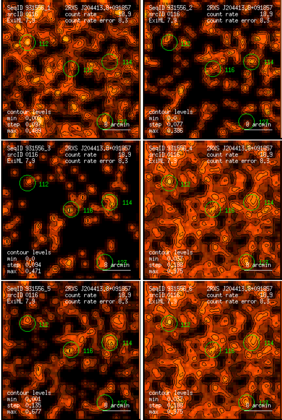
Figure 116: RASS 931556: detection 0116: band rate images, Gaussian filter: (1) PSPC channels 11 – 41, (2) 52 – 90, (3) 91 – 201, (4) 11 – 235, (5) 52 – 201, (6) 11 – 201. Broad band rates in counts/ks. Band rate contour levels in counts/ks/arcmin 2 .
