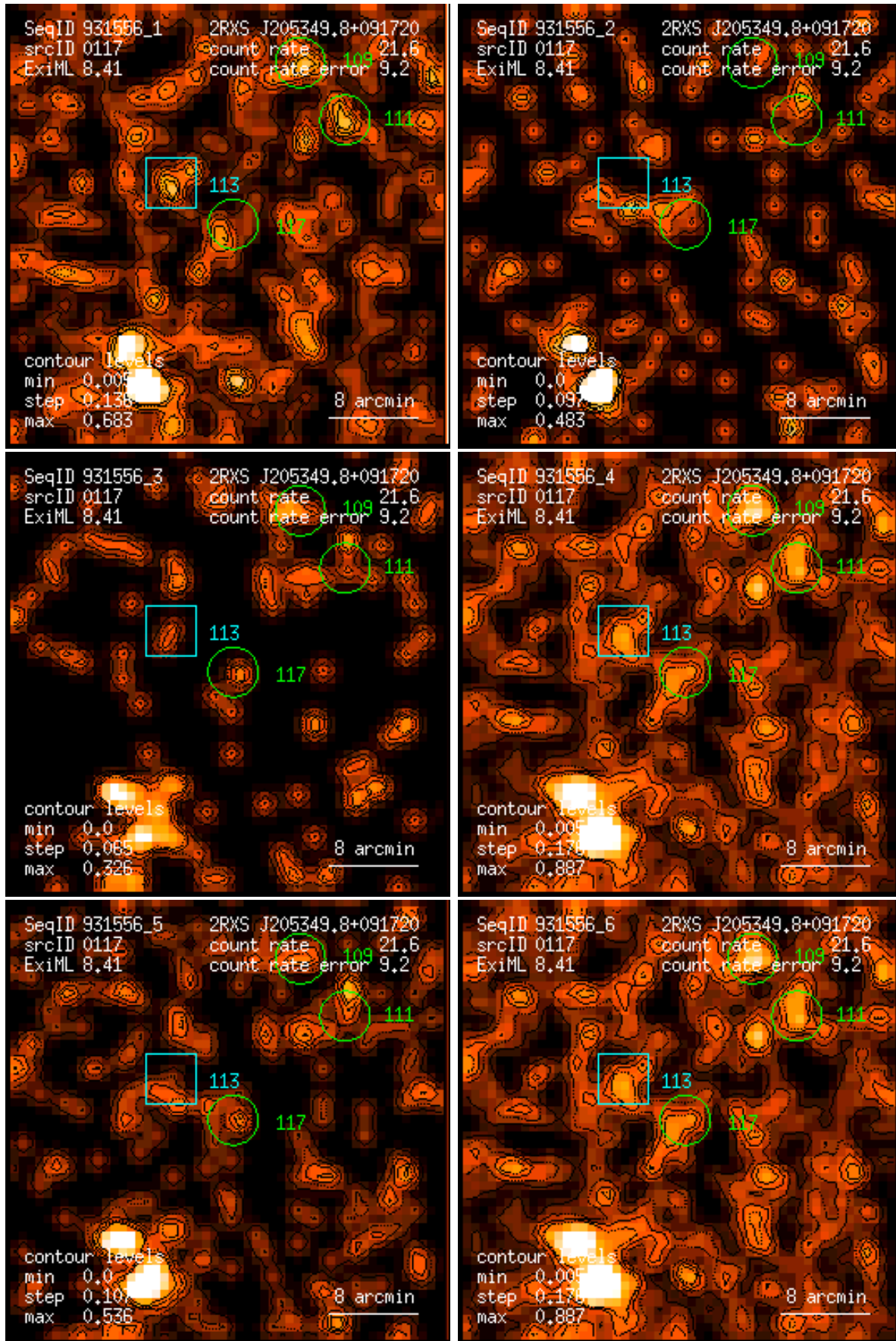
Figure 117: RASS 931556: detection 0117: band rate images, Gaussian filter: (1) PSPC channels 11 – 41, (2) 52 – 90, (3) 91 – 201, (4) 11 – 235, (5) 52 – 201, (6) 11 – 201. Broad band rates in counts/ks. Band rate contour levels in counts/ks/arcmin 2 .
