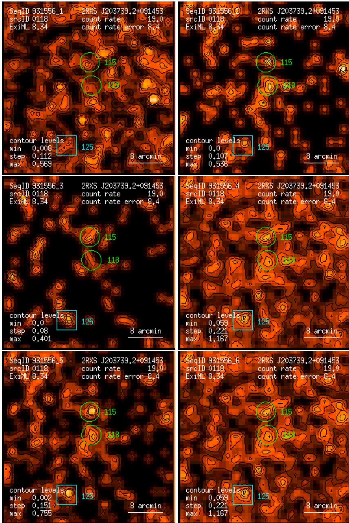
Figure 118: RASS 931556: detection 0118: band rate images, Gaussian filter: (1) PSPC channels 11 – 41, (2) 52 – 90, (3) 91 – 201, (4) 11 – 235, (5) 52 – 201, (6) 11 – 201. Broad band rates in counts/ks. Band rate contour levels in counts/ks/arcmin 2 .
