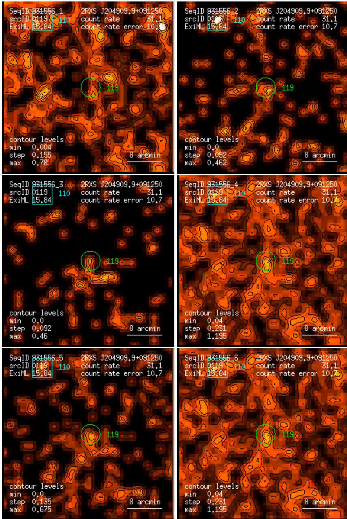
Figure 119: RASS 931556: detection 0119: band rate images, Gaussian filter: (1) PSPC channels 11 – 41, (2) 52 – 90, (3) 91 – 201, (4) 11 – 235, (5) 52 – 201, (6) 11 – 201. Broad band rates in counts/ks. Band rate contour levels in counts/ks/arcmin 2 .
