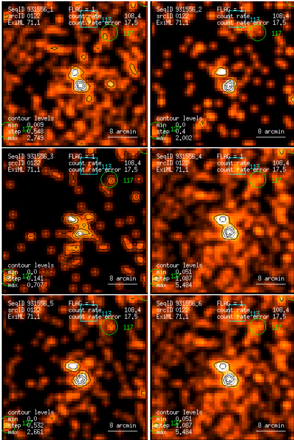
Figure 122: RASS 931556: detection 0122: band rate images, Gaussian filter: (1) PSPC channels 11 – 41, (2) 52 – 90, (3) 91 – 201, (4) 11 – 235, (5) 52 – 201, (6) 11 – 201. Broad band rates in counts/ks. Band rate contour levels in counts/ks/arcmin 2 .
