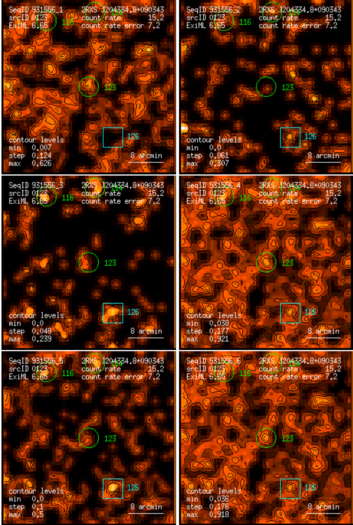
Figure 123: RASS 931556: detection 0123: band rate images, Gaussian filter: (1) PSPC channels 11 – 41, (2) 52 – 90, (3) 91 – 201, (4) 11 – 235, (5) 52 – 201, (6) 11 – 201. Broad band rates in counts/ks. Band rate contour levels in counts/ks/arcmin 2 .
