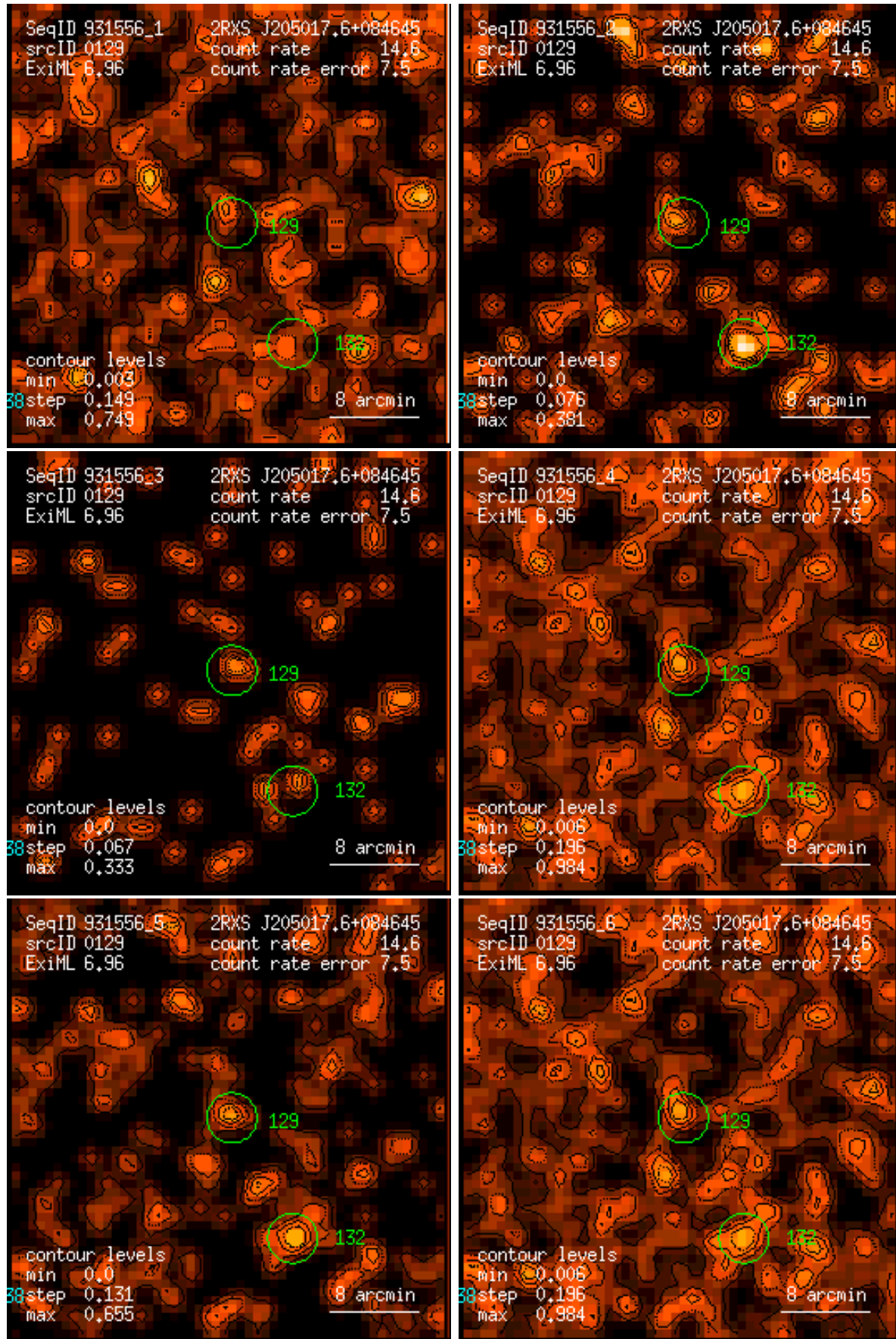
Figure 129: RASS 931556: detection 0129: band rate images, Gaussian filter: (1) PSPC channels 11 – 41, (2) 52 – 90, (3) 91 – 201, (4) 11 – 235, (5) 52 – 201, (6) 11 – 201. Broad band rates in counts/ks. Band rate contour levels in counts/ks/arcmin 2 .
