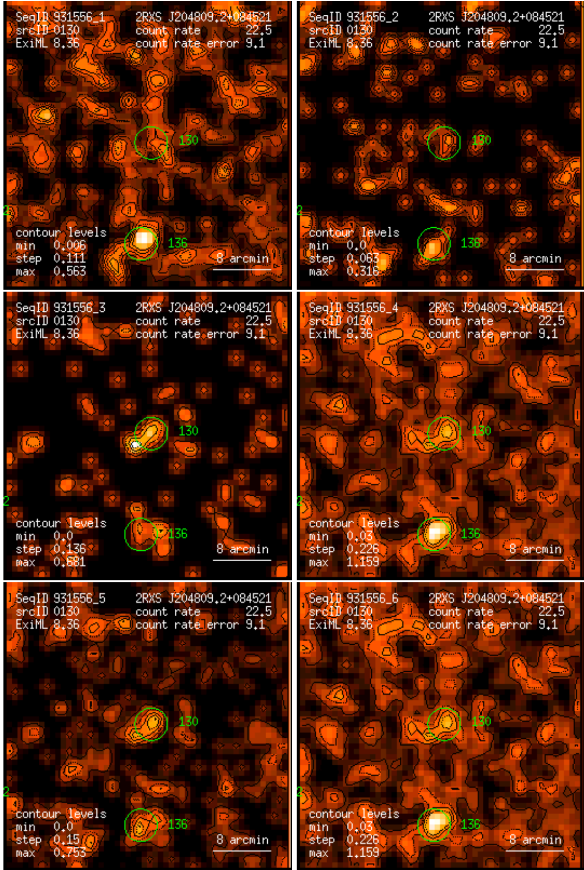
Figure 130: RASS 931556: detection 0130: band rate images, Gaussian filter: (1) PSPC channels 11 – 41, (2) 52 – 90, (3) 91 – 201, (4) 11 – 235, (5) 52 – 201, (6) 11 – 201. Broad band rates in counts/ks. Band rate contour levels in counts/ks/arcmin 2 .
