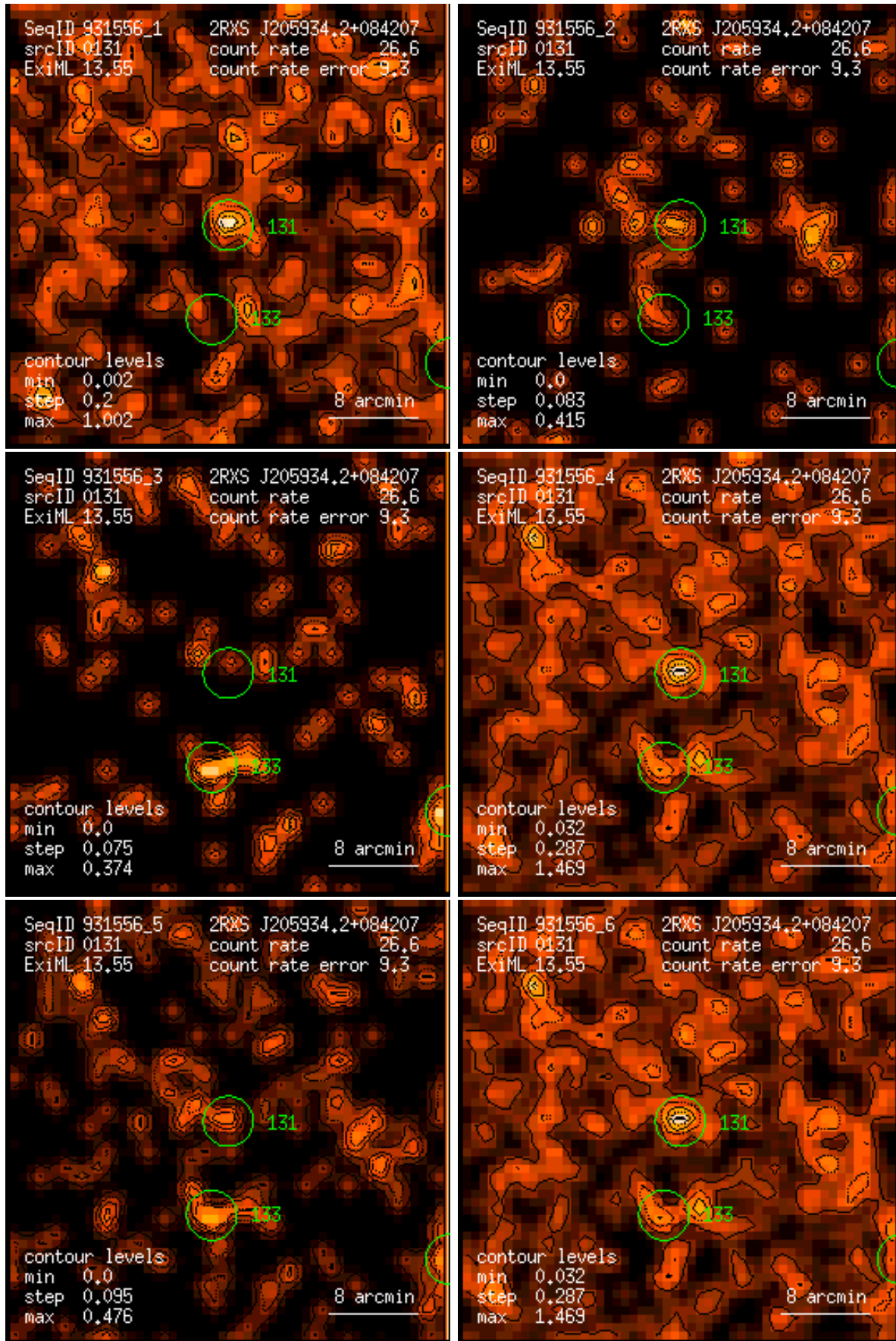
Figure 131: RASS 931556: detection 0131: band rate images, Gaussian filter: (1) PSPC channels 11 – 41, (2) 52 – 90, (3) 91 – 201, (4) 11 – 235, (5) 52 – 201, (6) 11 – 201. Broad band rates in counts/ks. Band rate contour levels in counts/ks/arcmin 2 .
