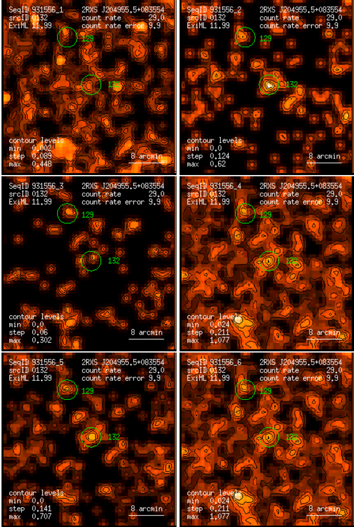
Figure 132: RASS 931556: detection 0132: band rate images, Gaussian filter: (1) PSPC channels 11 – 41, (2) 52 – 90, (3) 91 – 201, (4) 11 – 235, (5) 52 – 201, (6) 11 – 201. Broad band rates in counts/ks. Band rate contour levels in counts/ks/arcmin 2 .
