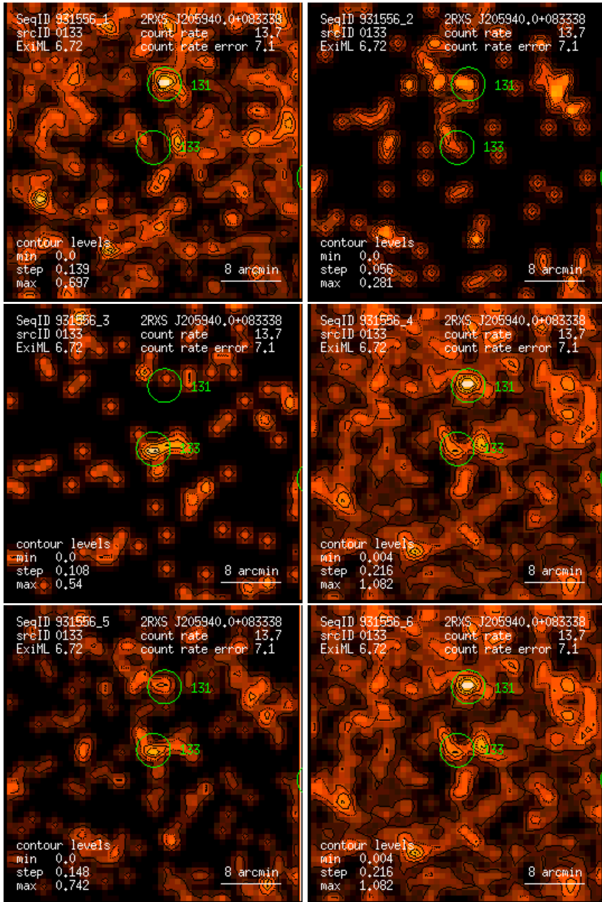
Figure 133: RASS 931556: detection 0133: band rate images, Gaussian filter: (1) PSPC channels 11 – 41, (2) 52 – 90, (3) 91 – 201, (4) 11 – 235, (5) 52 – 201, (6) 11 – 201. Broad band rates in counts/ks. Band rate contour levels in counts/ks/arcmin 2 .
