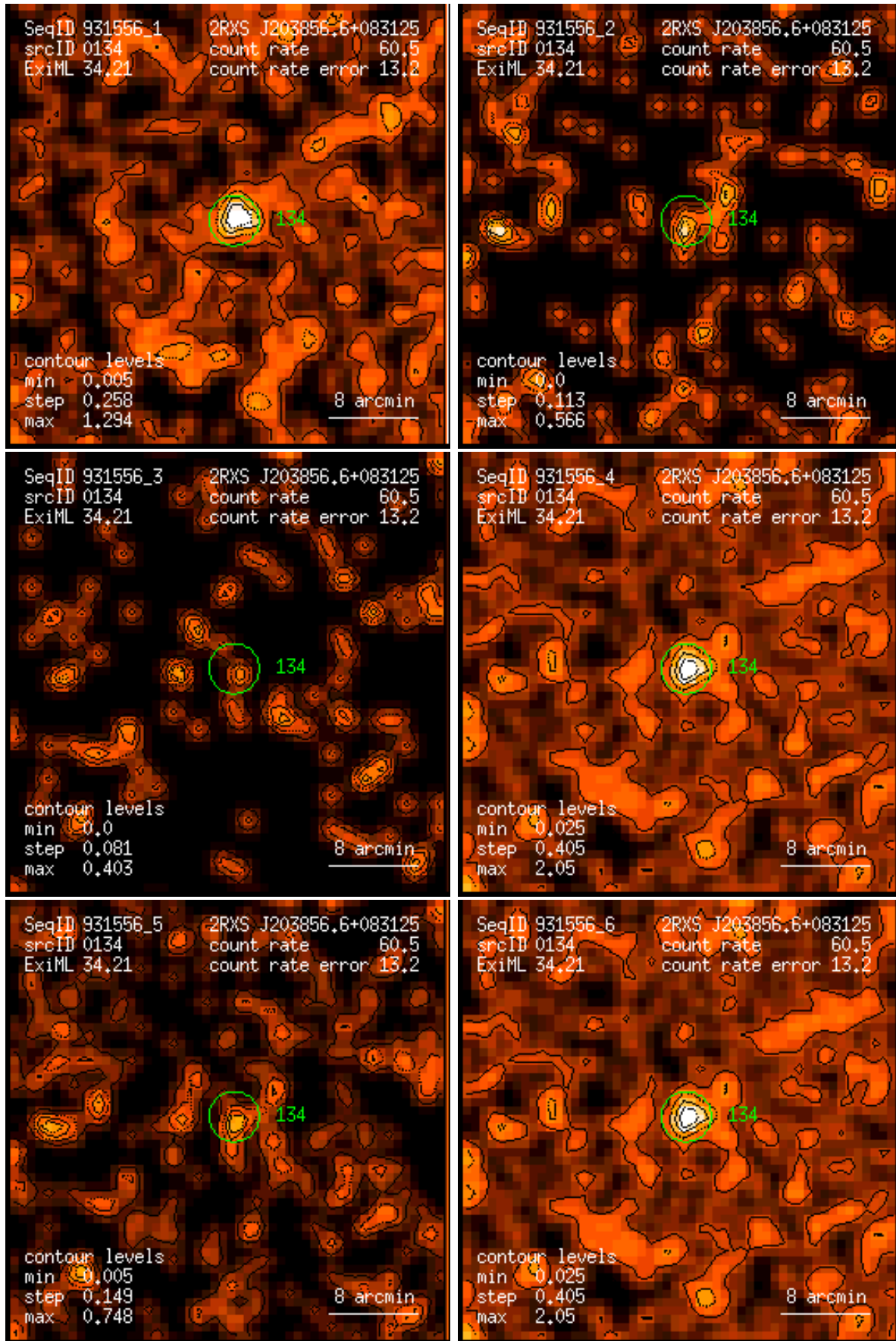
Figure 134: RASS 931556: detection 0134: band rate images, Gaussian filter: (1) PSPC channels 11 – 41, (2) 52 – 90, (3) 91 – 201, (4) 11 – 235, (5) 52 – 201, (6) 11 – 201. Broad band rates in counts/ks. Band rate contour levels in counts/ks/arcmin 2 .
