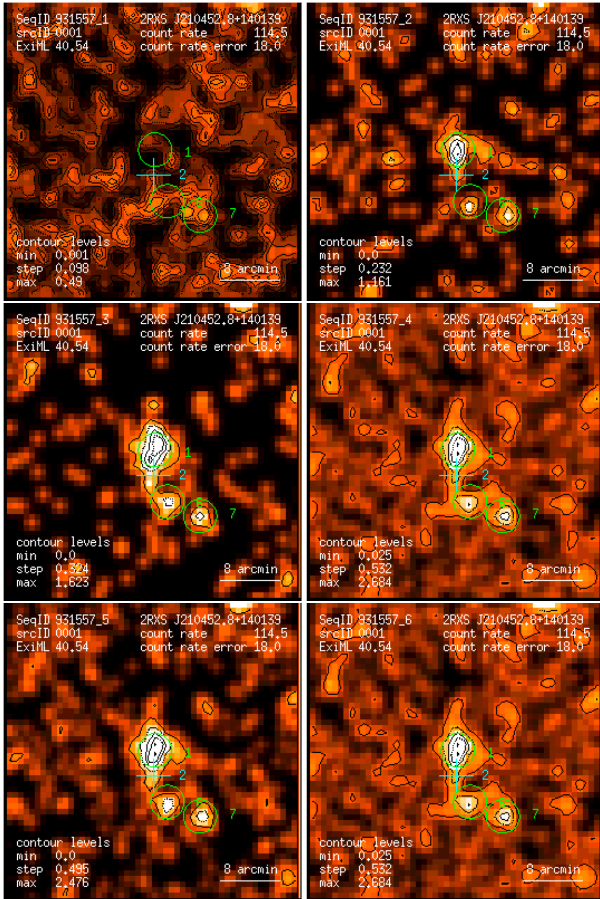
Figure 1: RASS 931557: detection 0001: band rate images, Gaussian filter: (1) PSPC channels 11 – 41, (2) 52 – 90, (3) 91 – 201, (4) 11 – 235, (5) 52 – 201, (6) 11 – 201. Broad band rates in counts/ks. Band rate contour levels in counts/ks/arcmin 2 .
