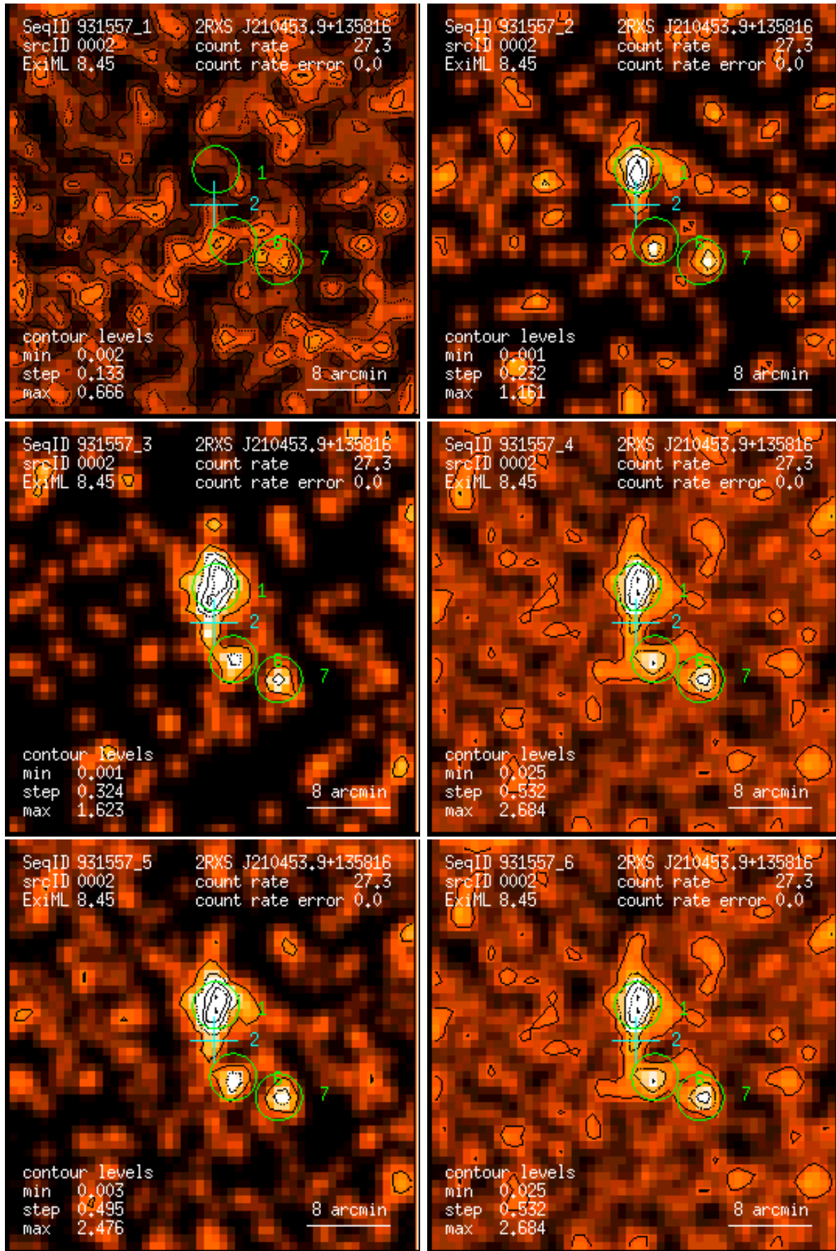
Figure 2: RASS 931557: detection 0002: band rate images, Gaussian filter: (1) PSPC channels 11 – 41, (2) 52 – 90, (3) 91 – 201, (4) 11 – 235, (5) 52 – 201, (6) 11 – 201. Broad band rates in counts/ks. Band rate contour levels in counts/ks/arcmin 2 .
