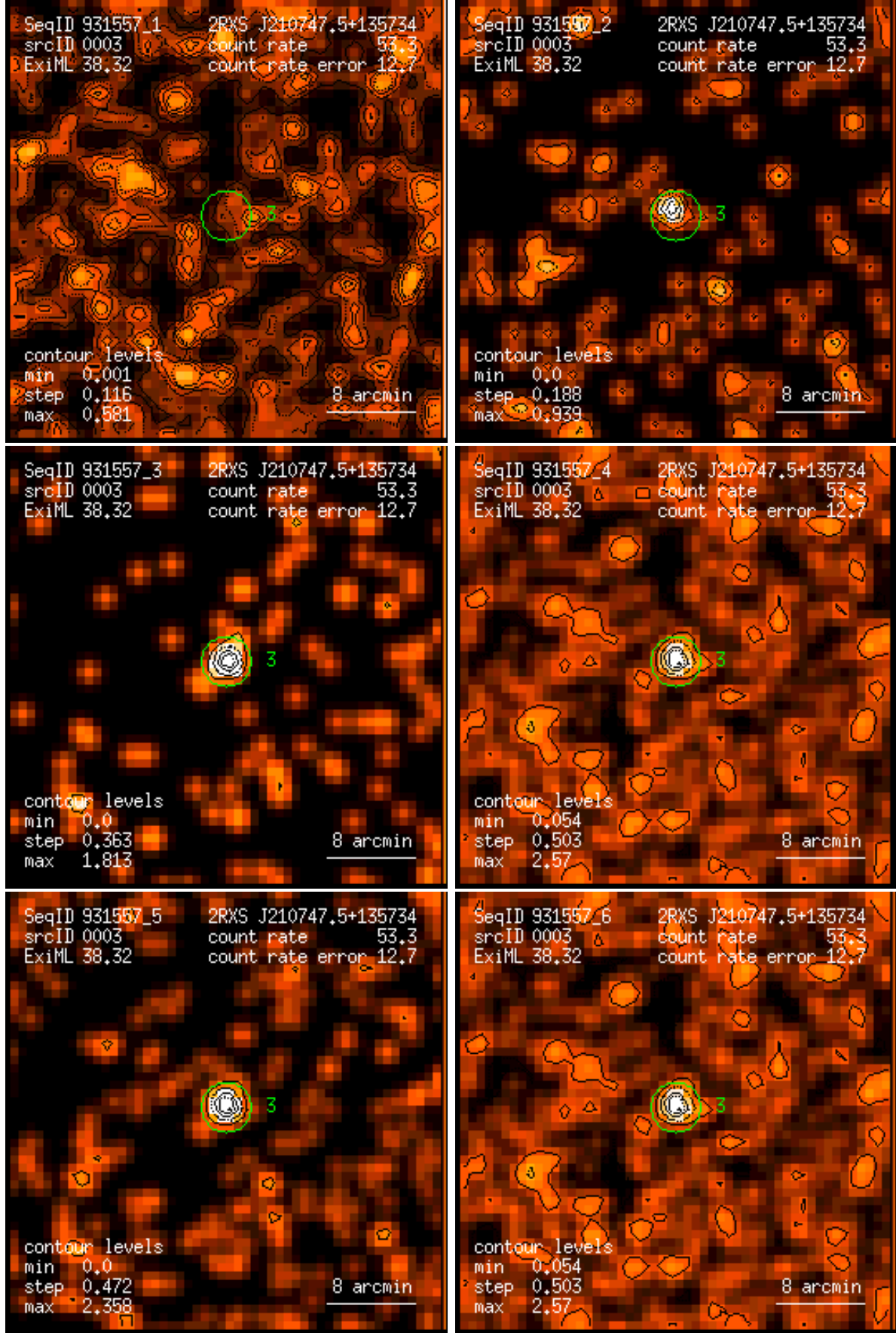
Figure 3: RASS 931557: detection 0003: band rate images, Gaussian filter: (1) PSPC channels 11 – 41, (2) 52 – 90, (3) 91 – 201, (4) 11 – 235, (5) 52 – 201, (6) 11 – 201. Broad band rates in counts/ks. Band rate contour levels in counts/ks/arcmin 2 .
