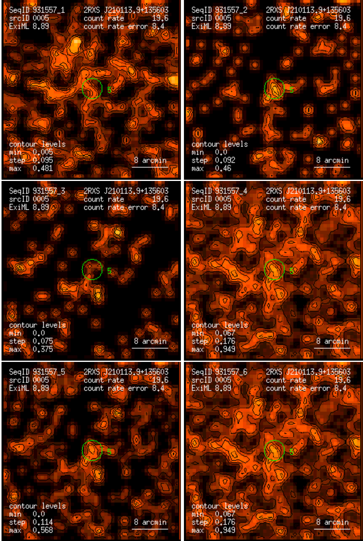
Figure 5: RASS 931557: detection 0005: band rate images, Gaussian filter: (1) PSPC channels 11 – 41, (2) 52 – 90, (3) 91 – 201, (4) 11 – 235, (5) 52 – 201, (6) 11 – 201. Broad band rates in counts/ks. Band rate contour levels in counts/ks/arcmin 2 .
