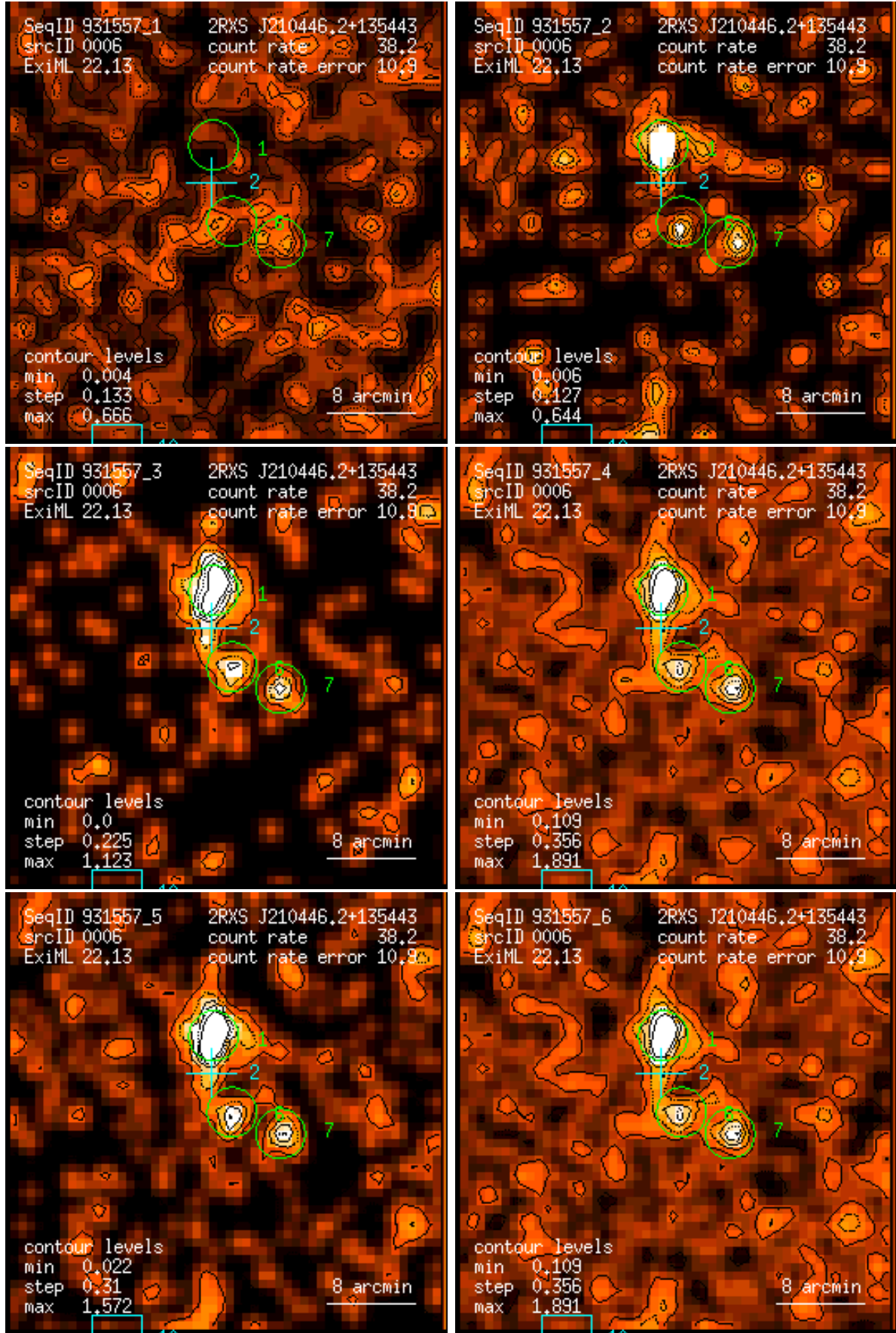
Figure 6: RASS 931557: detection 0006: band rate images, Gaussian filter: (1) PSPC channels 11 – 41, (2) 52 – 90, (3) 91 – 201, (4) 11 – 235, (5) 52 – 201, (6) 11 – 201. Broad band rates in counts/ks. Band rate contour levels in counts/ks/arcmin 2 .
