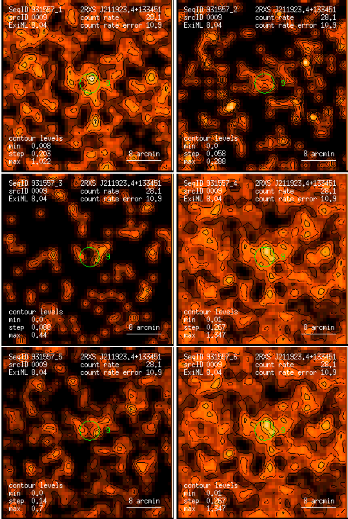
Figure 9: RASS 931557: detection 0009: band rate images, Gaussian filter: (1) PSPC channels 11 – 41, (2) 52 – 90, (3) 91 – 201, (4) 11 – 235, (5) 52 – 201, (6) 11 – 201. Broad band rates in counts/ks. Band rate contour levels in counts/ks/arcmin 2 .
