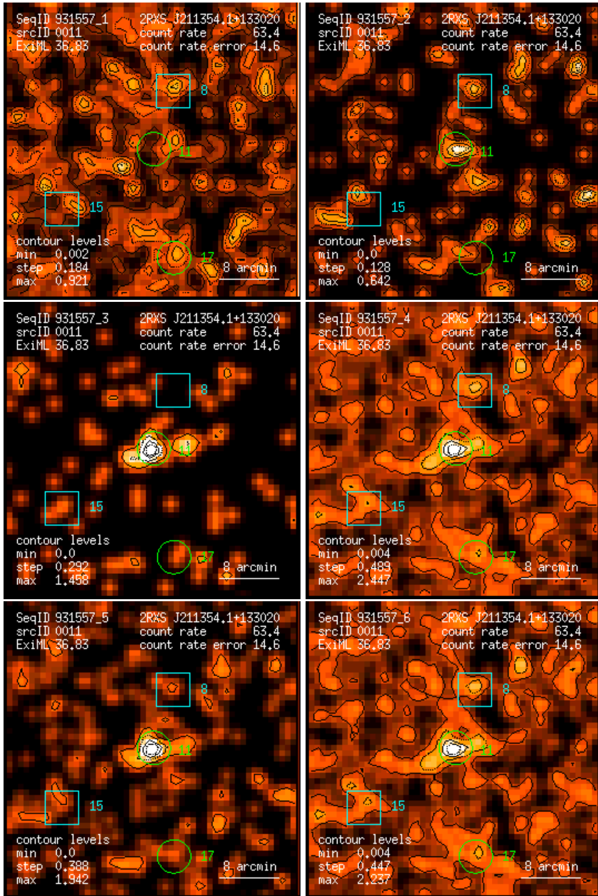
Figure 11: RASS 931557: detection 0011: band rate images, Gaussian filter: (1) PSPC channels 11 – 41, (2) 52 – 90, (3) 91 – 201, (4) 11 – 235, (5) 52 – 201, (6) 11 – 201. Broad band rates in counts/ks. Band rate contour levels in counts/ks/arcmin 2 .
