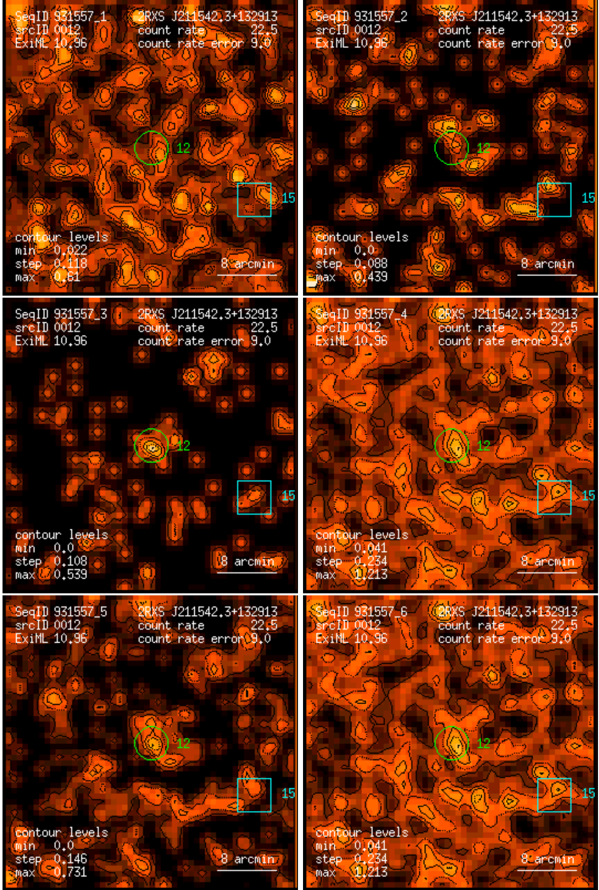
Figure 12: RASS 931557: detection 0012: band rate images, Gaussian filter: (1) PSPC channels 11 – 41, (2) 52 – 90, (3) 91 – 201, (4) 11 – 235, (5) 52 – 201, (6) 11 – 201. Broad band rates in counts/ks. Band rate contour levels in counts/ks/arcmin 2 .
