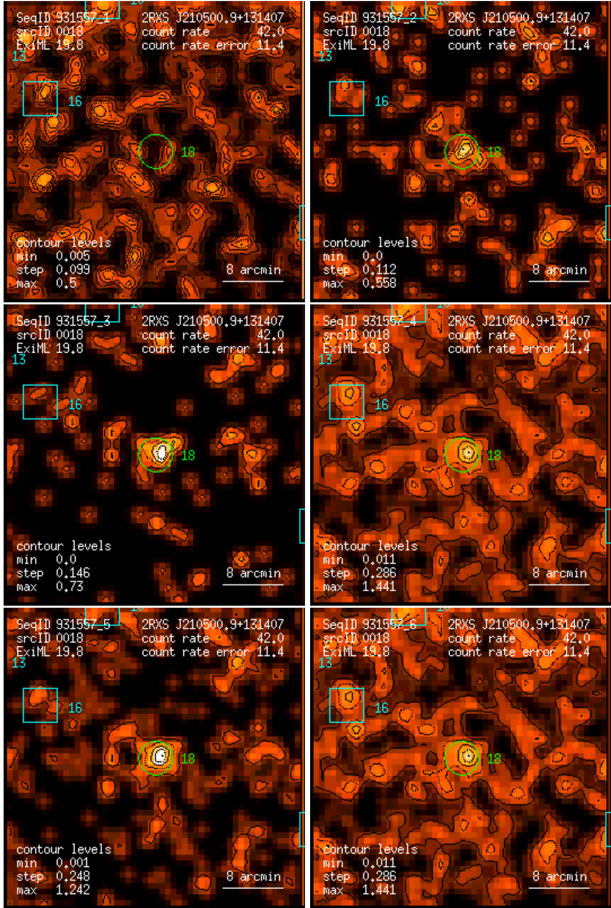
Figure 18: RASS 931557: detection 0018: band rate images, Gaussian filter: (1) PSPC channels 11 – 41, (2) 52 – 90, (3) 91 – 201, (4) 11 – 235, (5) 52 – 201, (6) 11 – 201. Broad band rates in counts/ks. Band rate contour levels in counts/ks/arcmin 2 .
