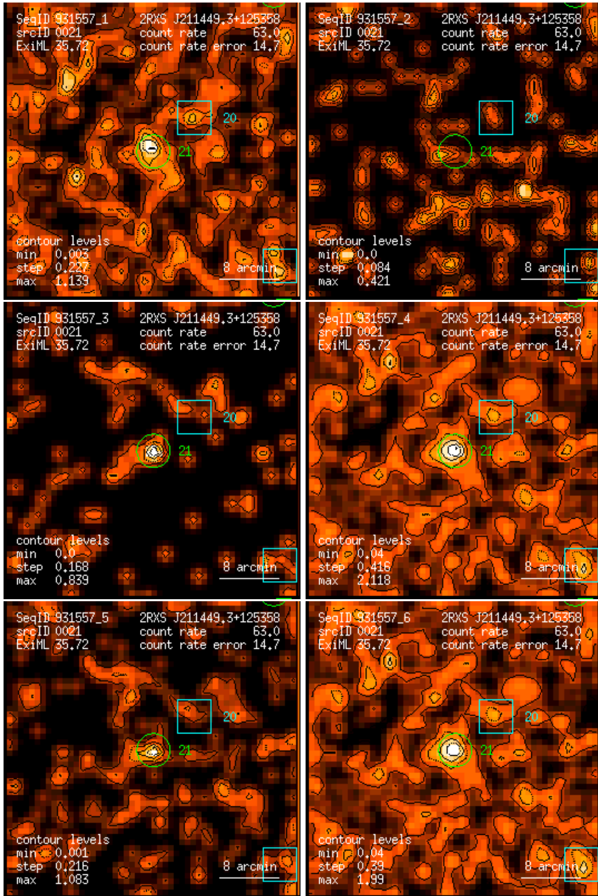
Figure 21: RASS 931557: detection 0021: band rate images, Gaussian filter: (1) PSPC channels 11 – 41, (2) 52 – 90, (3) 91 – 201, (4) 11 – 235, (5) 52 – 201, (6) 11 – 201. Broad band rates in counts/ks. Band rate contour levels in counts/ks/arcmin 2 .
