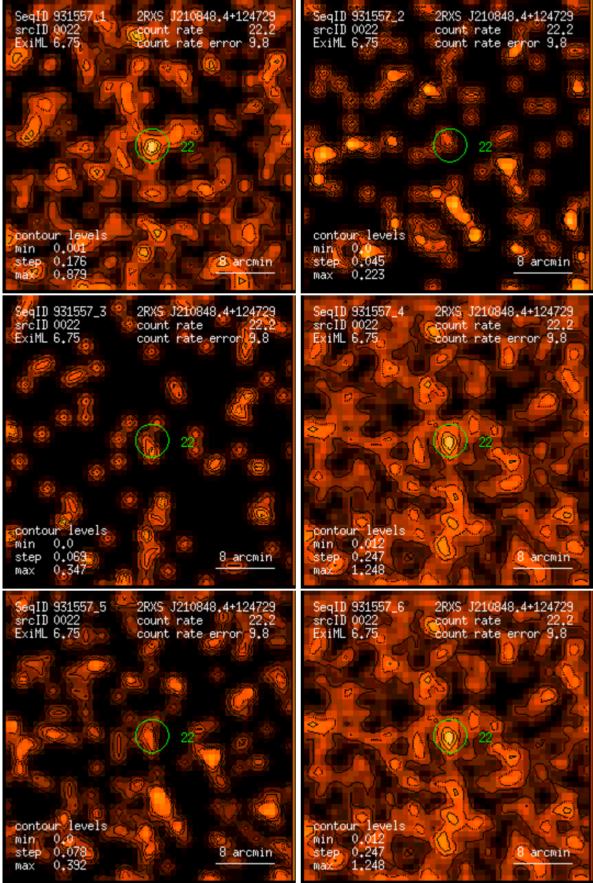
Figure 22: RASS 931557: detection 0022: band rate images, Gaussian filter: (1) PSPC channels 11 – 41, (2) 52 – 90, (3) 91 – 201, (4) 11 – 235, (5) 52 – 201, (6) 11 – 201. Broad band rates in counts/ks. Band rate contour levels in counts/ks/arcmin 2 .
