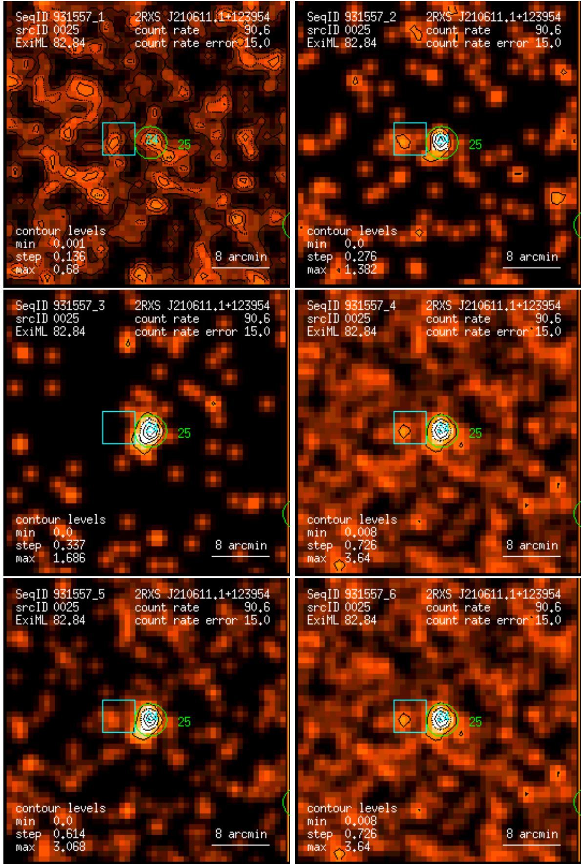
Figure 25: RASS 931557: detection 0025: band rate images, Gaussian filter: (1) PSPC channels 11 – 41, (2) 52 – 90, (3) 91 – 201, (4) 11 – 235, (5) 52 – 201, (6) 11 – 201. Broad band rates in counts/ks. Band rate contour levels in counts/ks/arcmin 2 .
