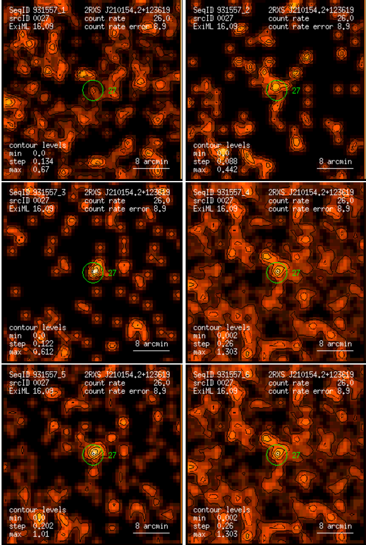
Figure 27: RASS 931557: detection 0027: band rate images, Gaussian filter: (1) PSPC channels 11 – 41, (2) 52 – 90, (3) 91 – 201, (4) 11 – 235, (5) 52 – 201, (6) 11 – 201. Broad band rates in counts/ks. Band rate contour levels in counts/ks/arcmin 2 .
