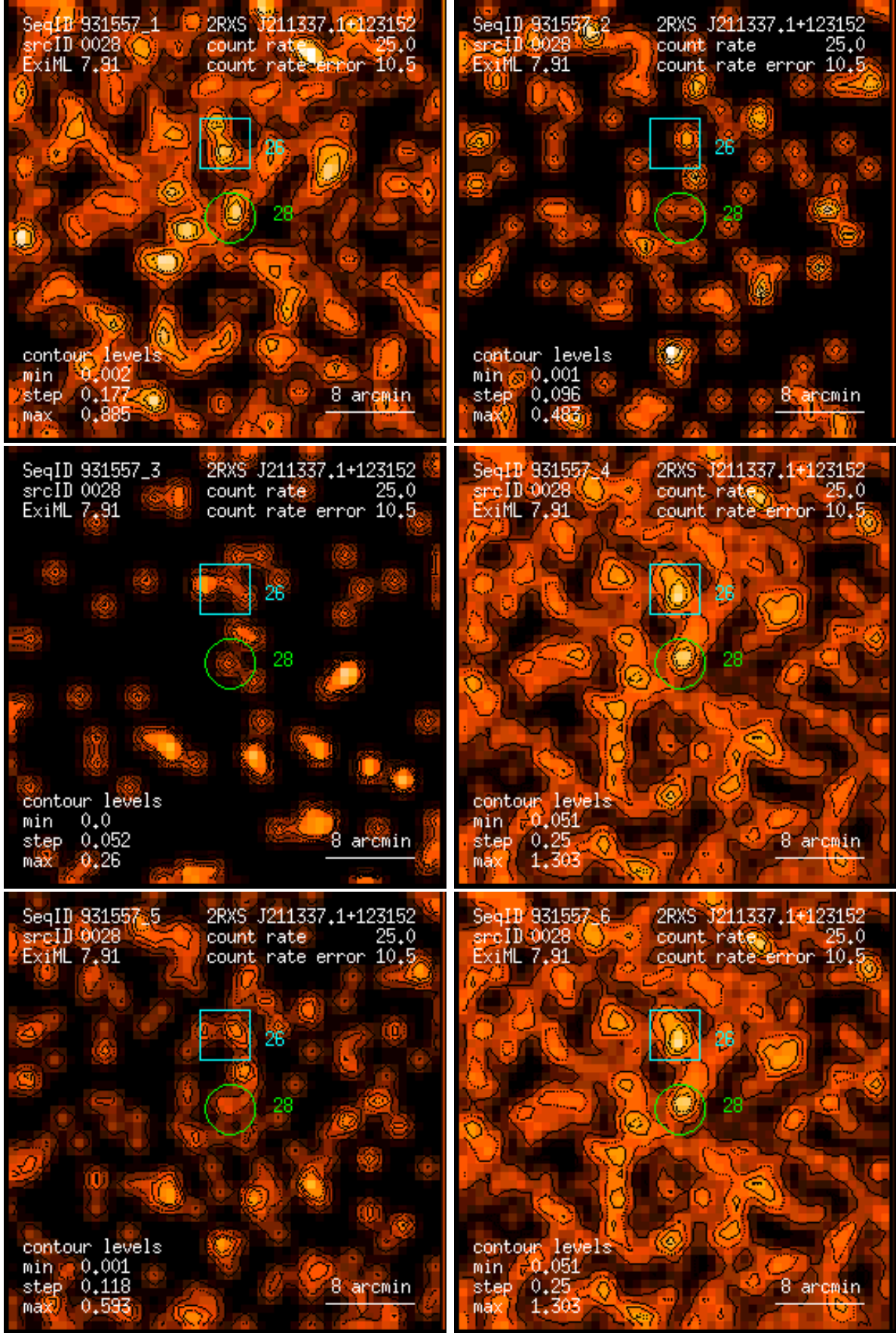
Figure 28: RASS 931557: detection 0028: band rate images, Gaussian filter: (1) PSPC channels 11 – 41, (2) 52 – 90, (3) 91 – 201, (4) 11 – 235, (5) 52 – 201, (6) 11 – 201. Broad band rates in counts/ks. Band rate contour levels in counts/ks/arcmin 2 .
