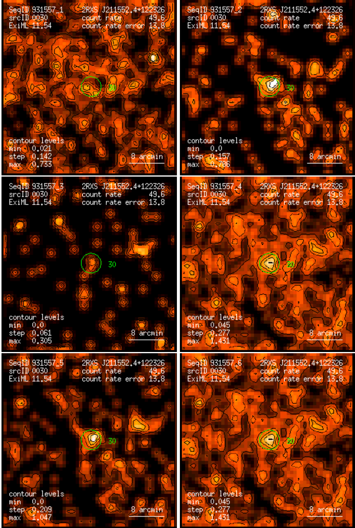
Figure 30: RASS 931557: detection 0030: band rate images, Gaussian filter: (1) PSPC channels 11 – 41, (2) 52 – 90, (3) 91 – 201, (4) 11 – 235, (5) 52 – 201, (6) 11 – 201. Broad band rates in counts/ks. Band rate contour levels in counts/ks/arcmin 2 .
