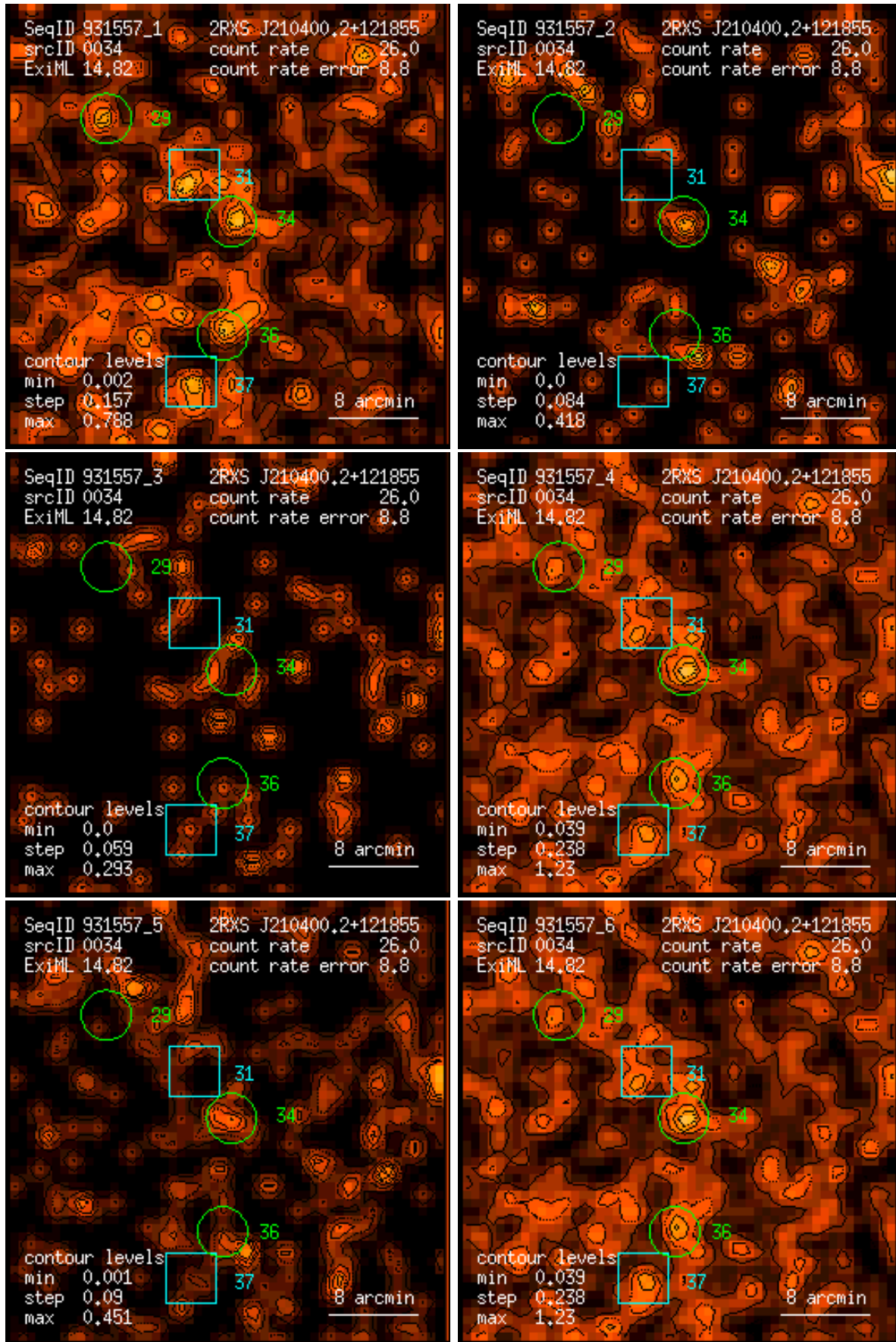
Figure 34: RASS 931557: detection 0034: band rate images, Gaussian filter: (1) PSPC channels 11 – 41, (2) 52 – 90, (3) 91 – 201, (4) 11 – 235, (5) 52 – 201, (6) 11 – 201. Broad band rates in counts/ks. Band rate contour levels in counts/ks/arcmin 2 .
