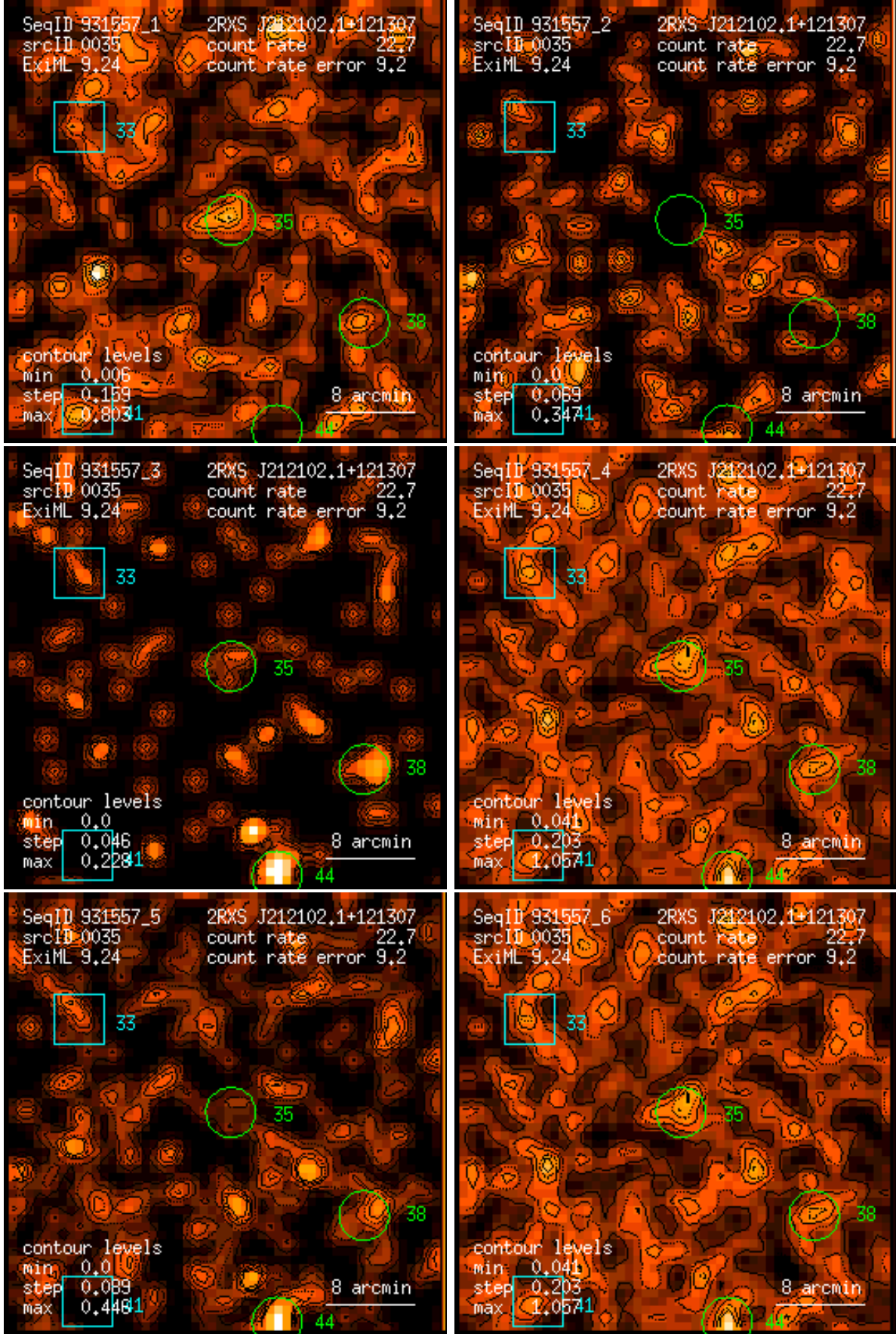
Figure 35: RASS 931557: detection 0035: band rate images, Gaussian filter: (1) PSPC channels 11 – 41, (2) 52 – 90, (3) 91 – 201, (4) 11 – 235, (5) 52 – 201, (6) 11 – 201. Broad band rates in counts/ks. Band rate contour levels in counts/ks/arcmin 2 .
