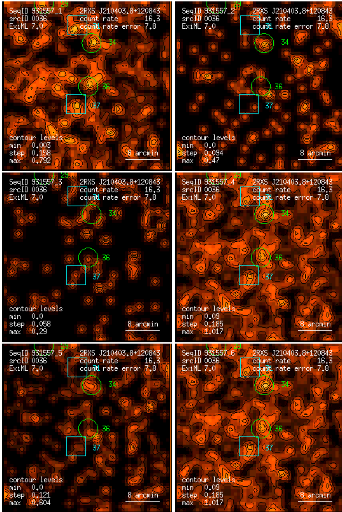
Figure 36: RASS 931557: detection 0036: band rate images, Gaussian filter: (1) PSPC channels 11 – 41, (2) 52 – 90, (3) 91 – 201, (4) 11 – 235, (5) 52 – 201, (6) 11 – 201. Broad band rates in counts/ks. Band rate contour levels in counts/ks/arcmin 2 .
