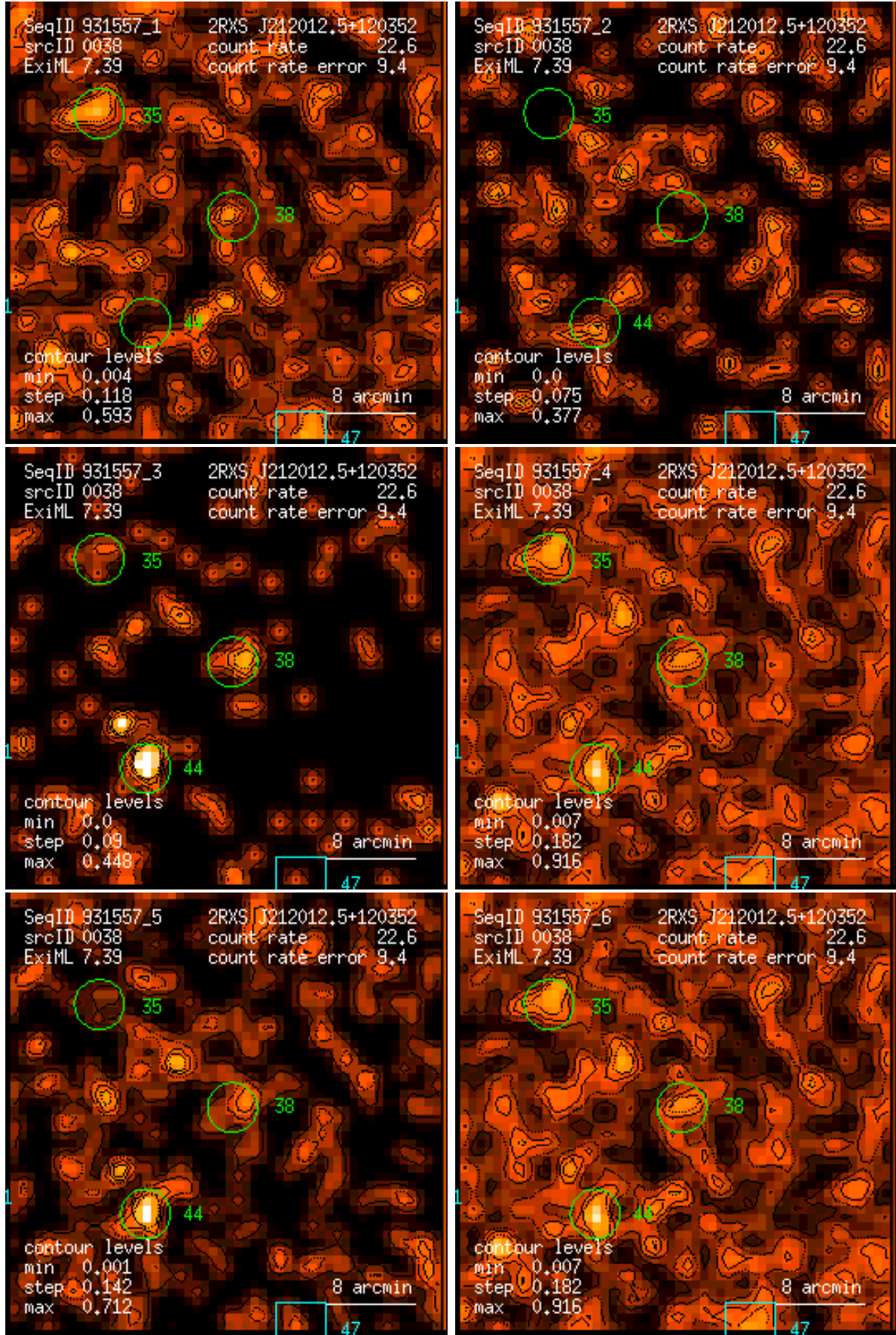
Figure 38: RASS 931557: detection 0038: band rate images, Gaussian filter: (1) PSPC channels 11 – 41, (2) 52 – 90, (3) 91 – 201, (4) 11 – 235, (5) 52 – 201, (6) 11 – 201. Broad band rates in counts/ks. Band rate contour levels in counts/ks/arcmin 2 .
