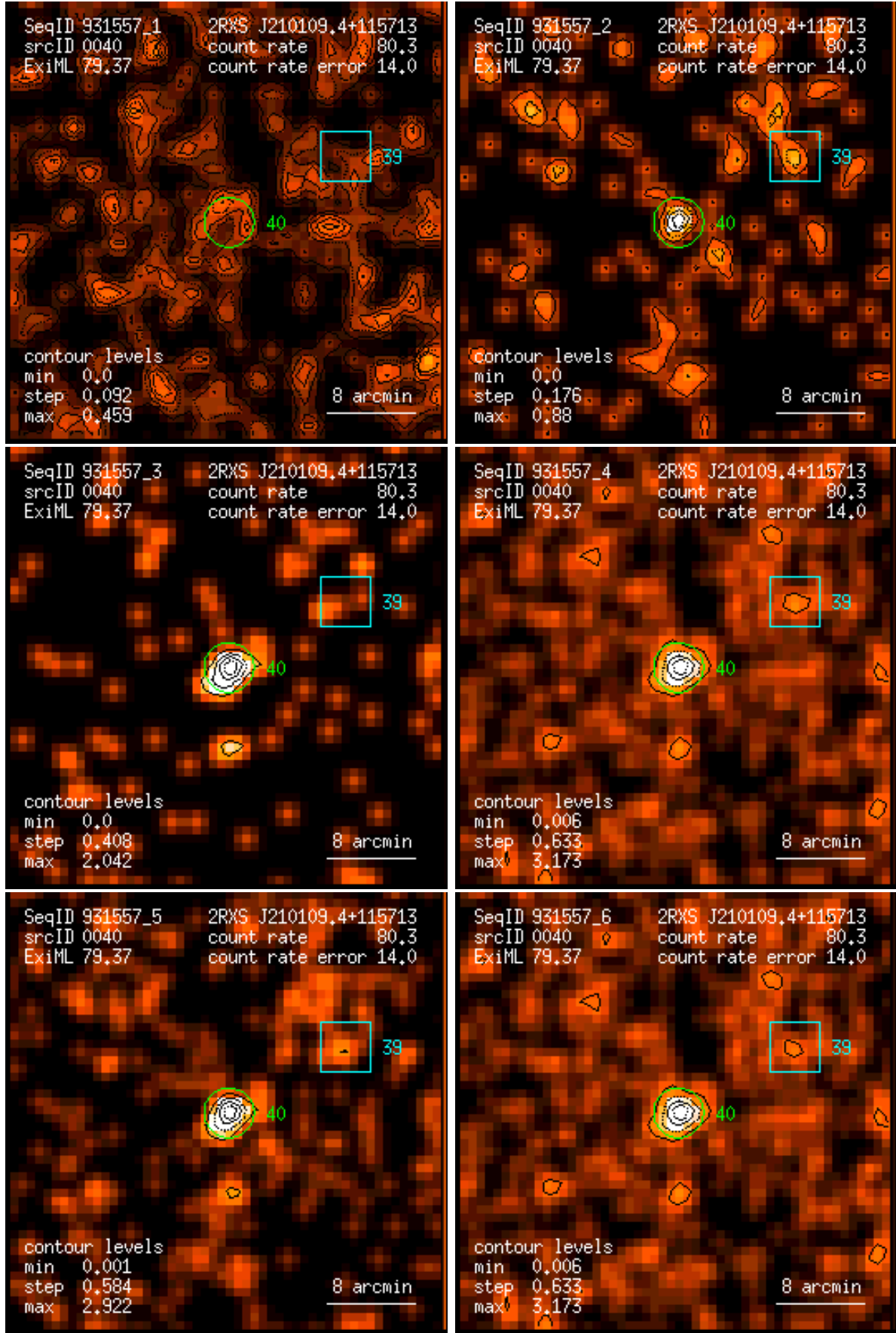
Figure 40: RASS 931557: detection 0040: band rate images, Gaussian filter: (1) PSPC channels 11 – 41, (2) 52 – 90, (3) 91 – 201, (4) 11 – 235, (5) 52 – 201, (6) 11 – 201. Broad band rates in counts/ks. Band rate contour levels in counts/ks/arcmin 2 .
