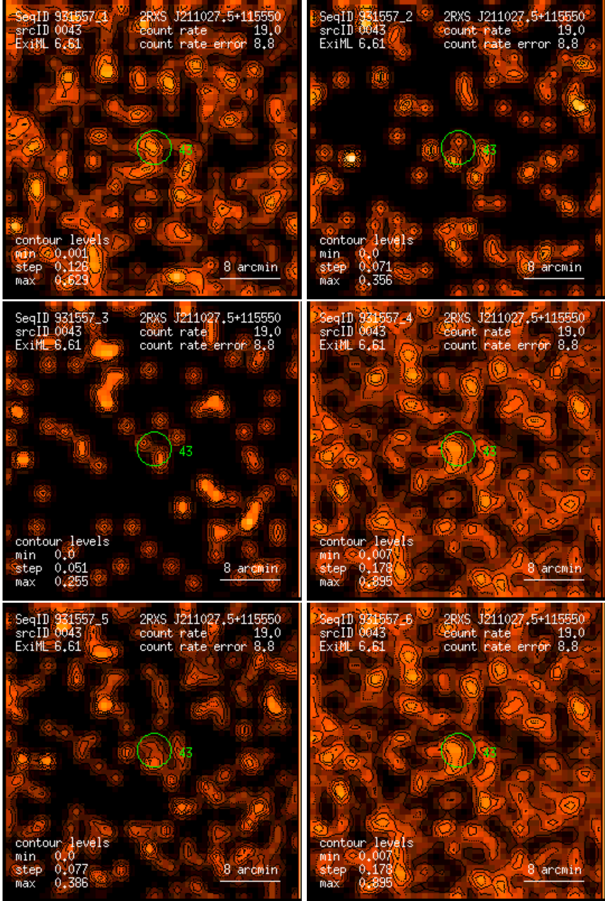
Figure 43: RASS 931557: detection 0043: band rate images, Gaussian filter: (1) PSPC channels 11 – 41, (2) 52 – 90, (3) 91 – 201, (4) 11 – 235, (5) 52 – 201, (6) 11 – 201. Broad band rates in counts/ks. Band rate contour levels in counts/ks/arcmin 2 .
