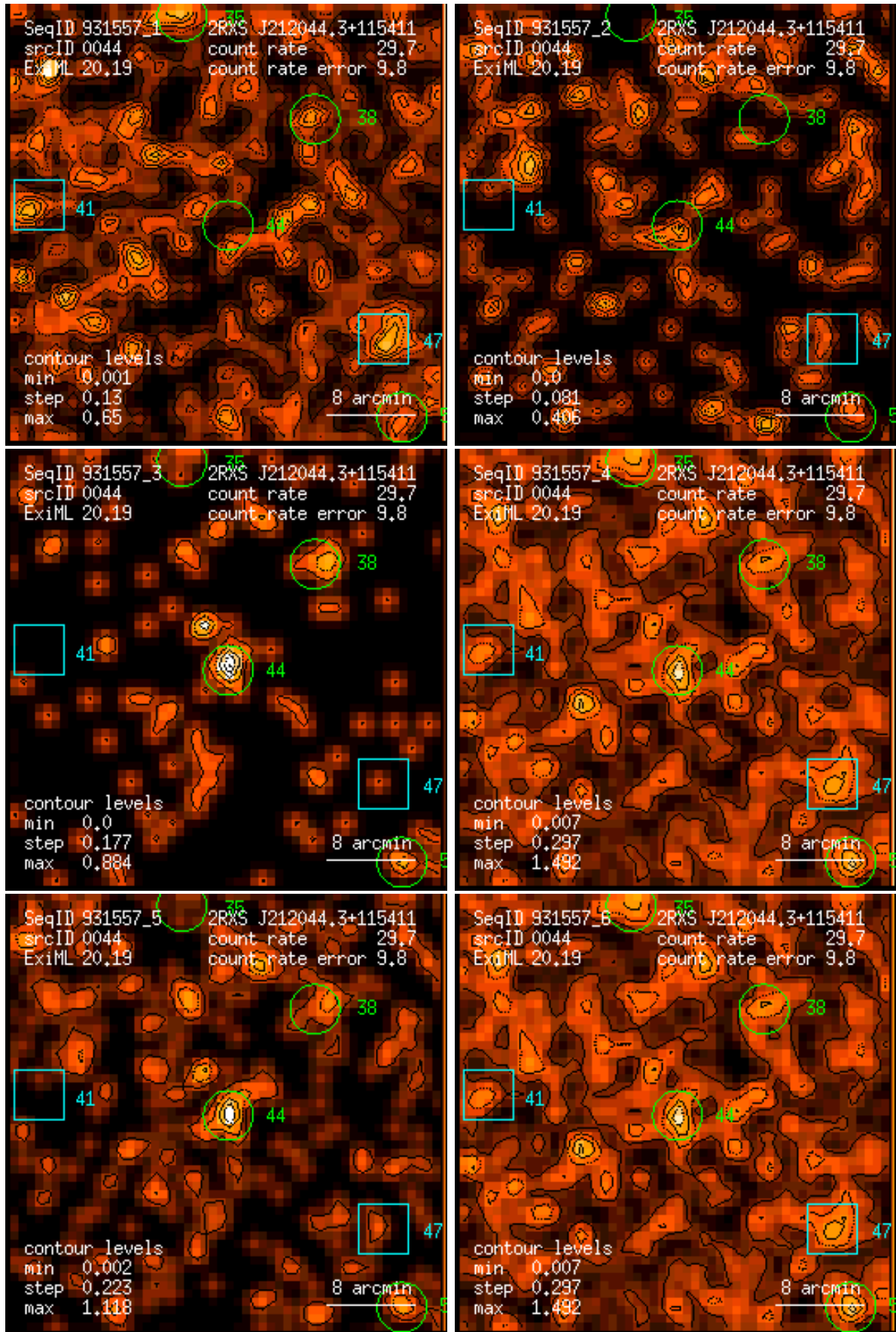
Figure 44: RASS 931557: detection 0044: band rate images, Gaussian filter: (1) PSPC channels 11 – 41, (2) 52 – 90, (3) 91 – 201, (4) 11 – 235, (5) 52 – 201, (6) 11 – 201. Broad band rates in counts/ks. Band rate contour levels in counts/ks/arcmin 2 .
