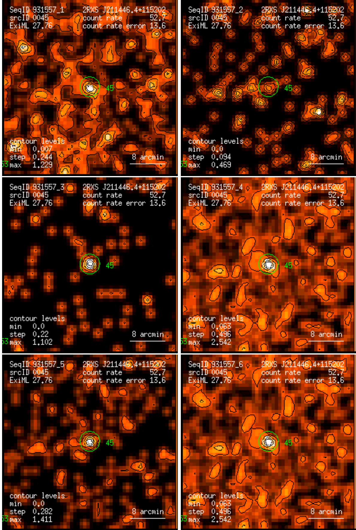
Figure 45: RASS 931557: detection 0045: band rate images, Gaussian filter: (1) PSPC channels 11 – 41, (2) 52 – 90, (3) 91 – 201, (4) 11 – 235, (5) 52 – 201, (6) 11 – 201. Broad band rates in counts/ks. Band rate contour levels in counts/ks/arcmin 2 .
