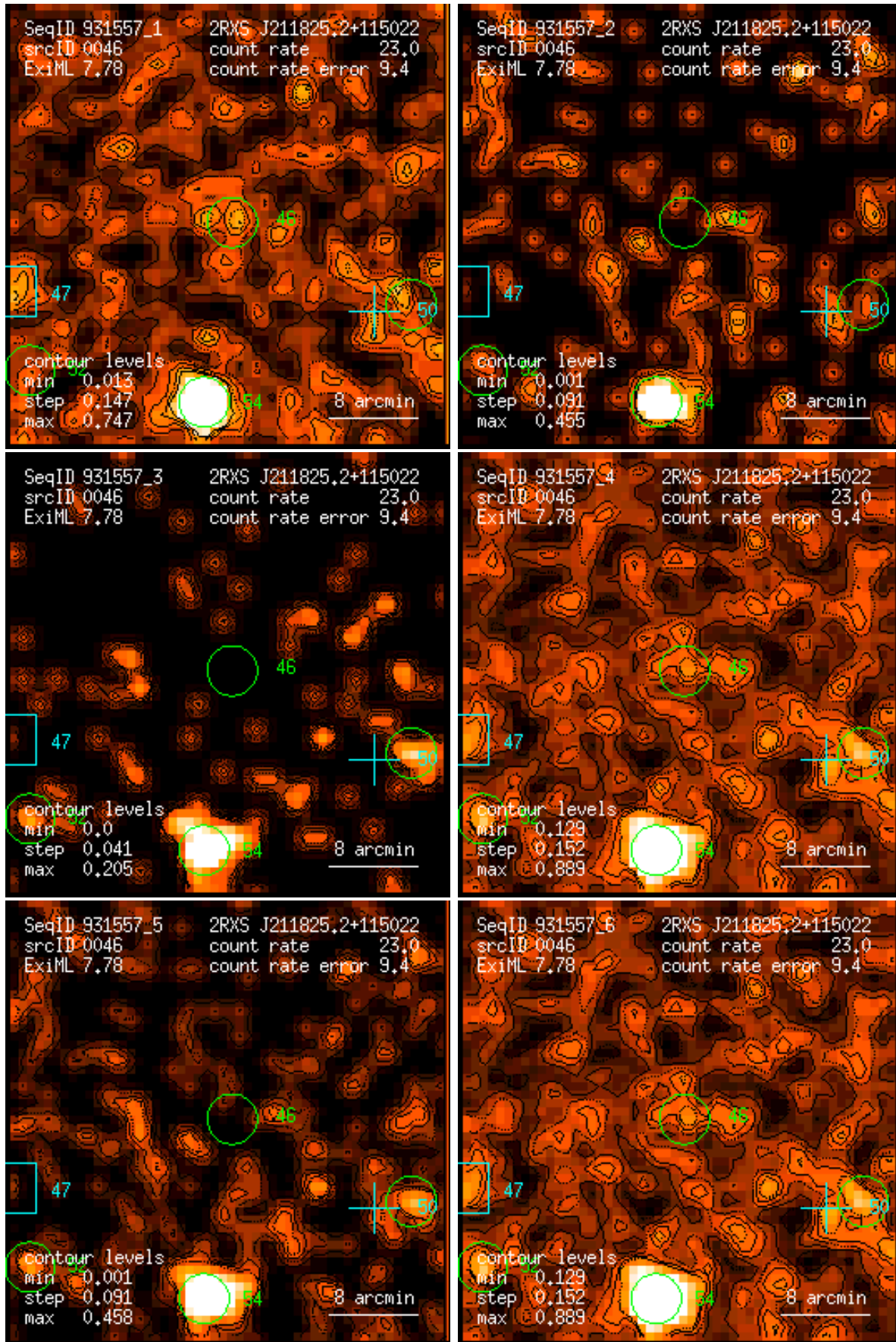
Figure 46: RASS 931557: detection 0046: band rate images, Gaussian filter: (1) PSPC channels 11 – 41, (2) 52 – 90, (3) 91 – 201, (4) 11 – 235, (5) 52 – 201, (6) 11 – 201. Broad band rates in counts/ks. Band rate contour levels in counts/ks/arcmin 2 .
